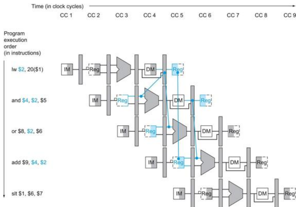
FIGURE 4.58 A pipelined sequence of instructions.
