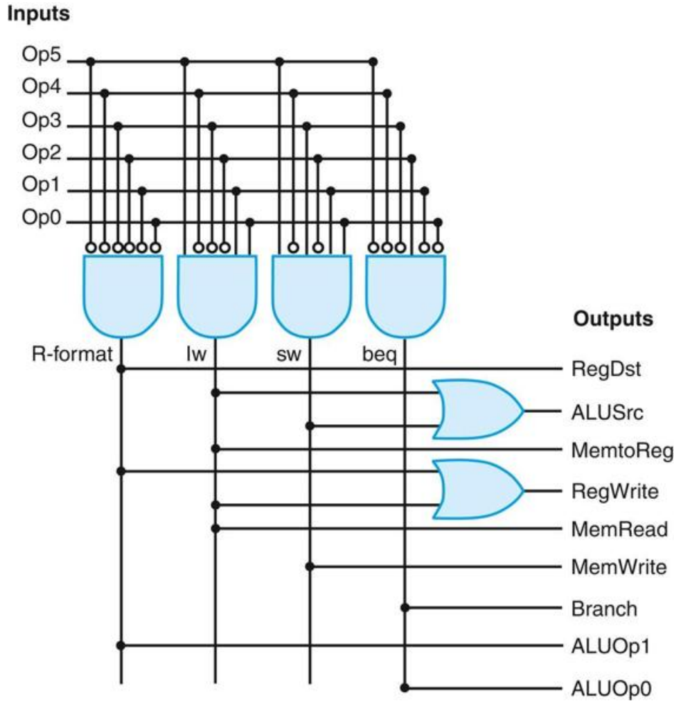
FIGURE D.2.5 The structured implementation of the control function as described by the truth table in Figure D.2.4 .
