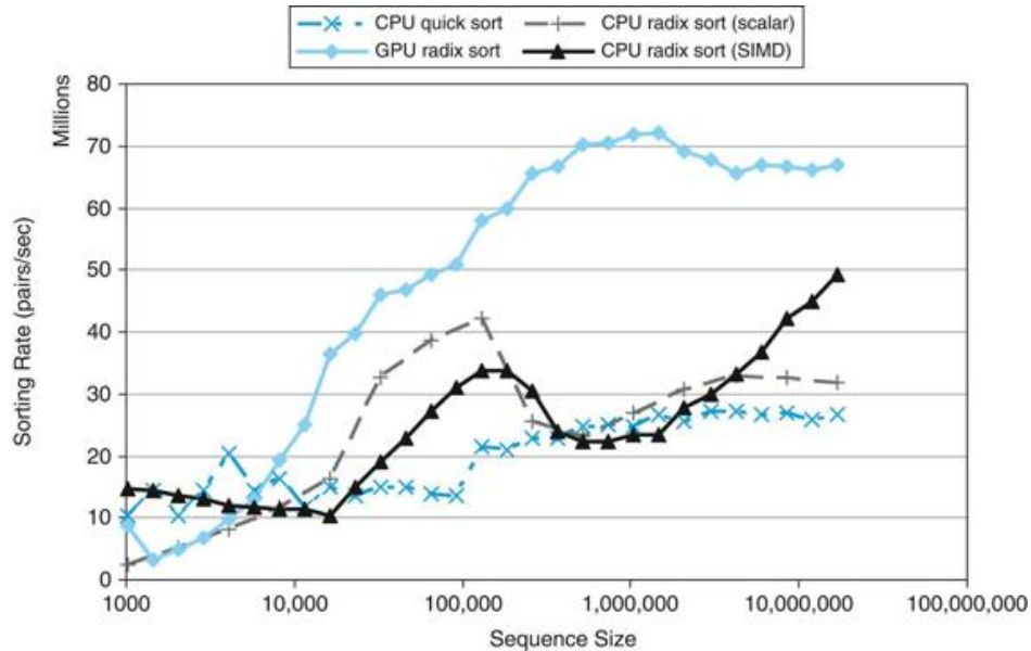
FIGURE C.7.6 Parallel sorting performance.
