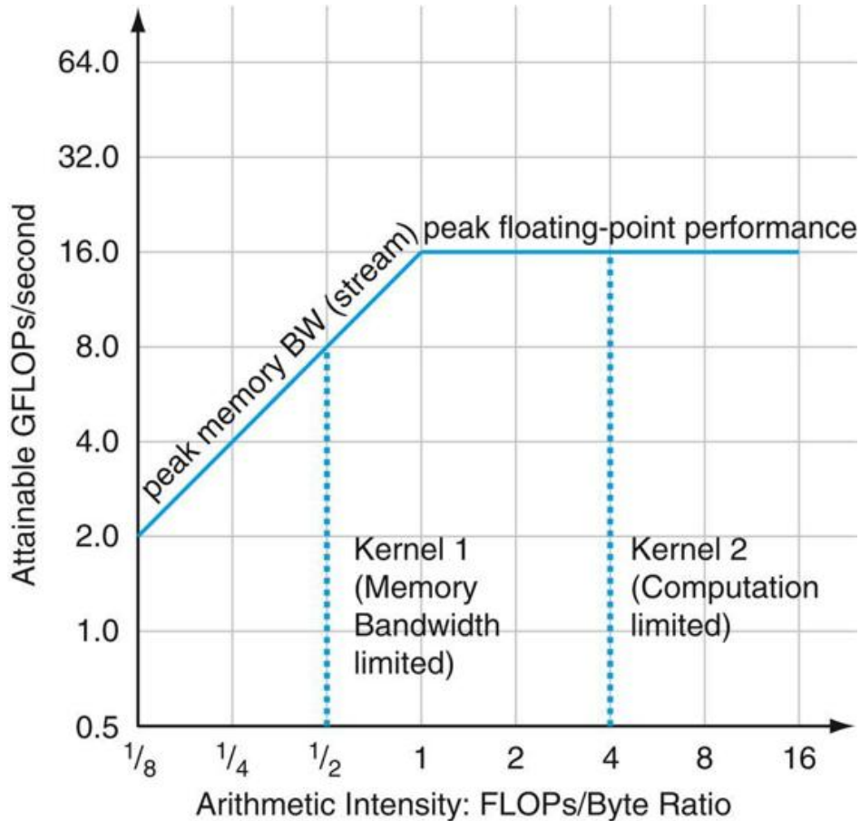
FIGURE 6.19 Roofline Model [Williams, Waterman, and Patterson, 2009].
