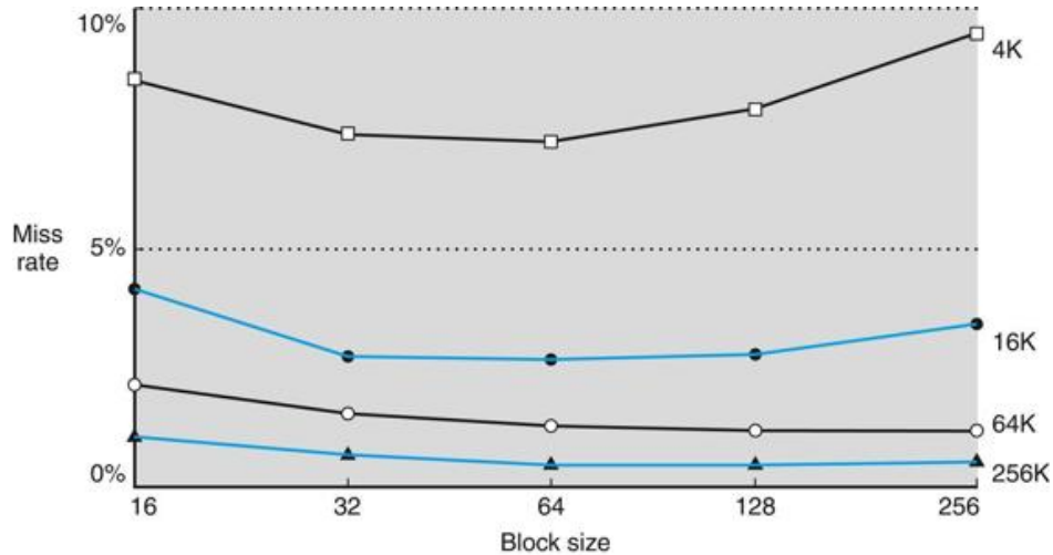
FIGURE 5.11 Miss rate versus block size.
