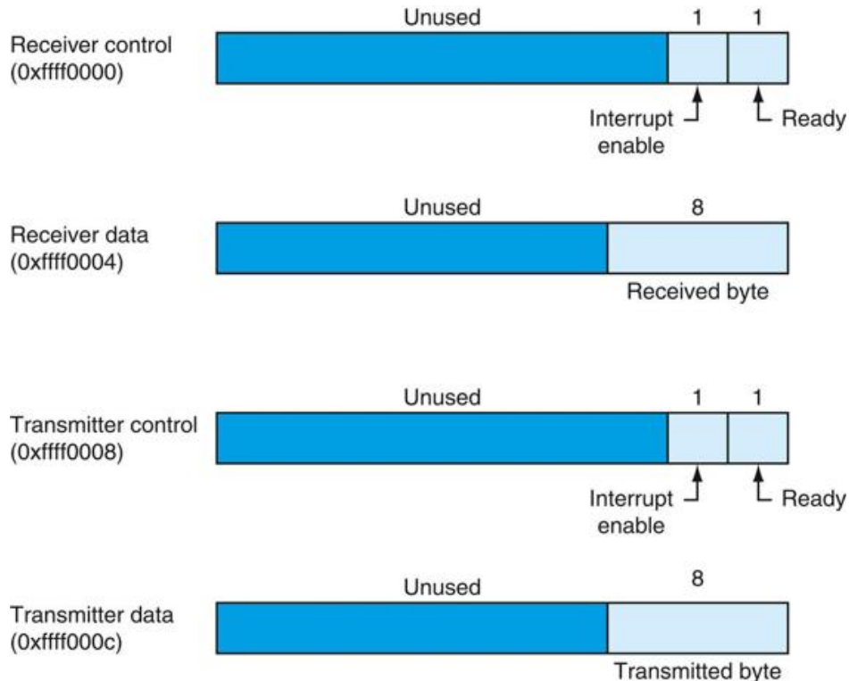
FIGURE A.8.1 The terminal is controlled by four device registers, each of which appears as a memory location at the given address.
