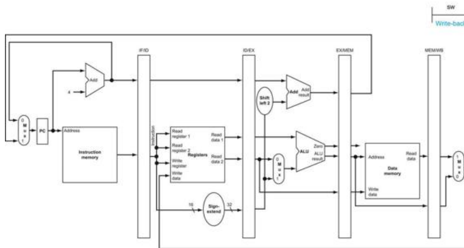
FIGURE 4.40 MEM and WB: The fourth and fifth pipe stages of a store instruction.
