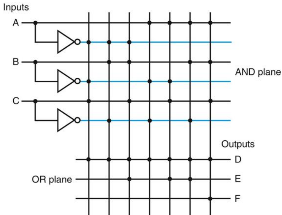
FIGURE B.3.5 A PLA drawn using dots to indicate the components of the product terms and sum terms in the array.
