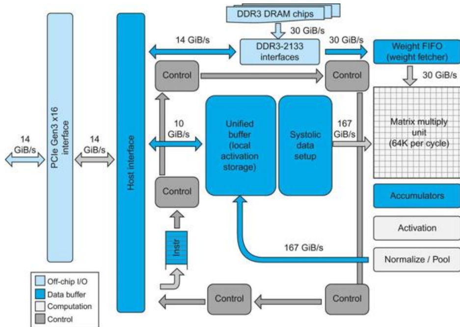
FIGURE 6.13 TPUv1 Block Diagram.
