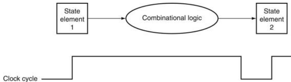
FIGURE B.7.2 The inputs to a combinational logic block come from a state element, and the outputs are written into a state element.
