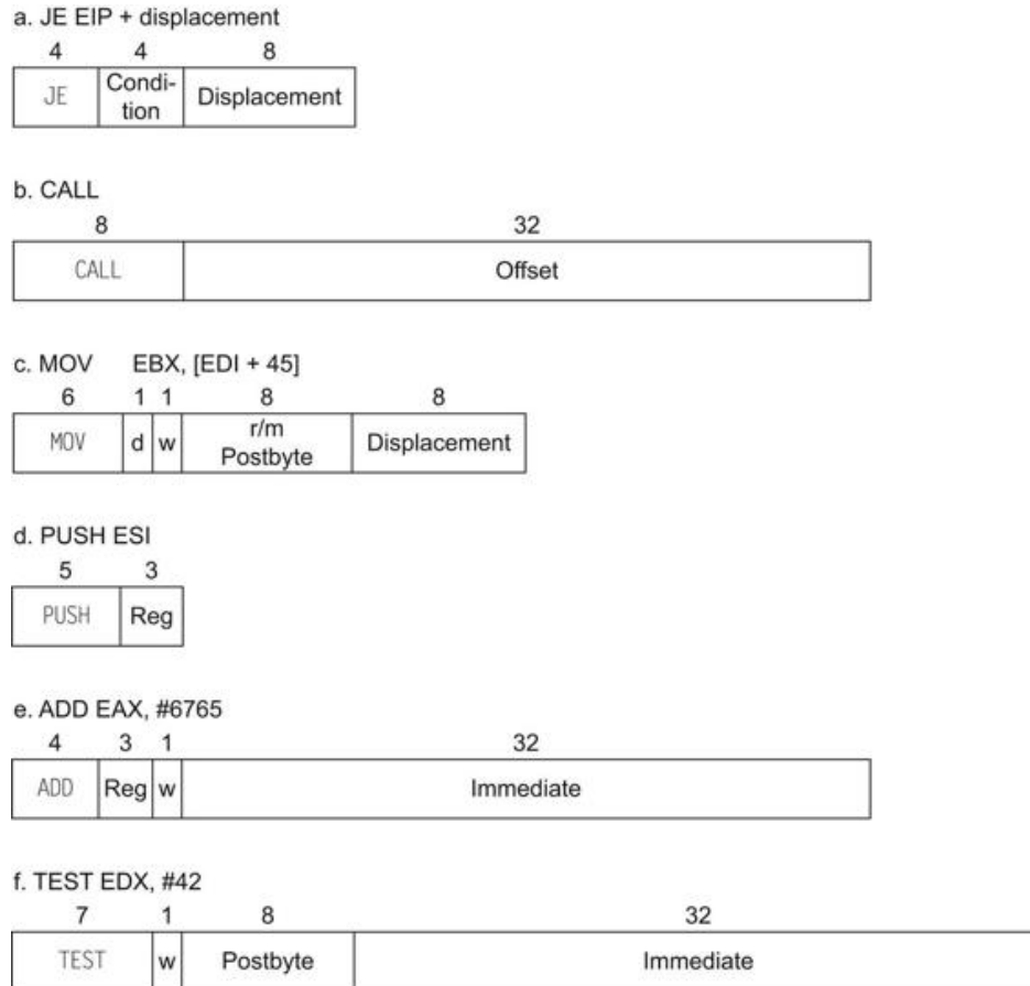
FIGURE 2.41 Typical x86 instruction formats.
