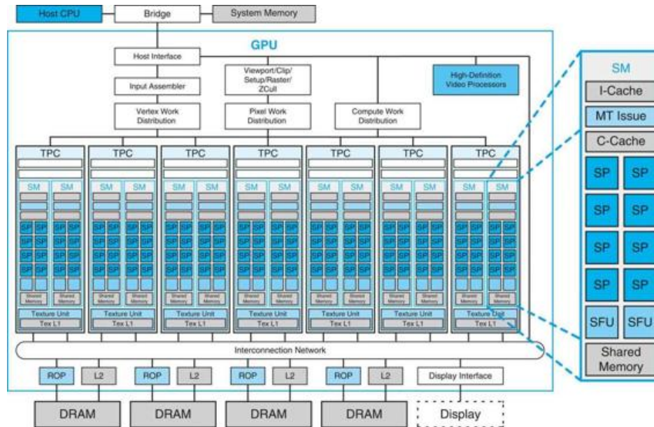
FIGURE C.2.5 Basic unified GPU architecture.
