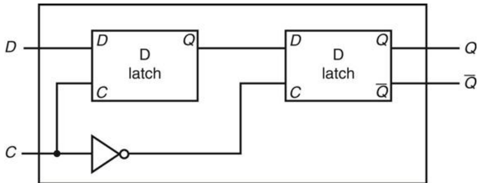
FIGURE B.8.4 A D flip-flop with a falling-edge trigger.
