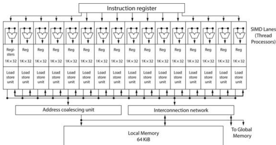
FIGURE 6.9 Simplified block diagram of the datapath of a multithreaded SIMD Processor.
