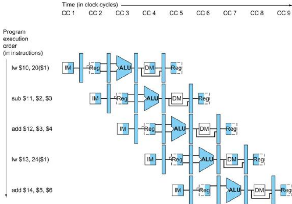
FIGURE 4.43 Multiple-clock-cycle pipeline diagram of five instructions.
