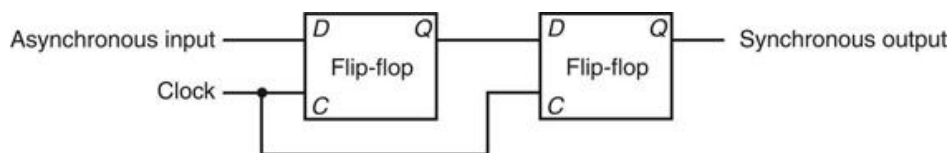
FIGURE B.11.6 This synchronizer will work correctly if the period of metastability that we wish to guard against is less than the clock period.
