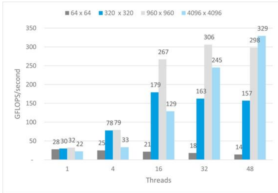
FIGURE 6.33 DGEMM performance versus the number of threads for four matrix sizes.
