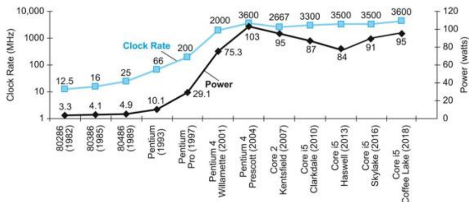
FIGURE 1.16 Clock rate and Power for Intel x86 microprocessors over nine generations and 36 years.
