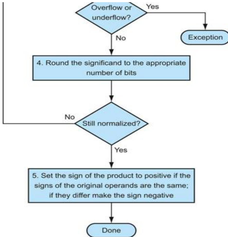
FIGURE 3.16 Floating-point multiplication. The normal path is to execute steps 3 and 4 once, but if rounding causes the sum to be unnormalized, we must repeat step 3.
