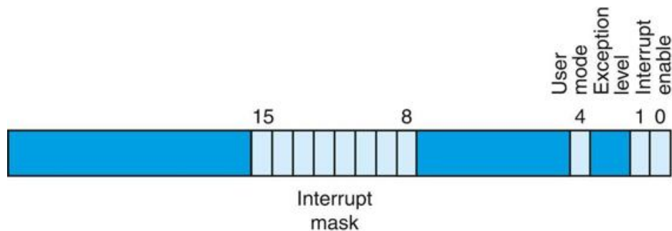
FIGURE A.7.1 The Status register.
