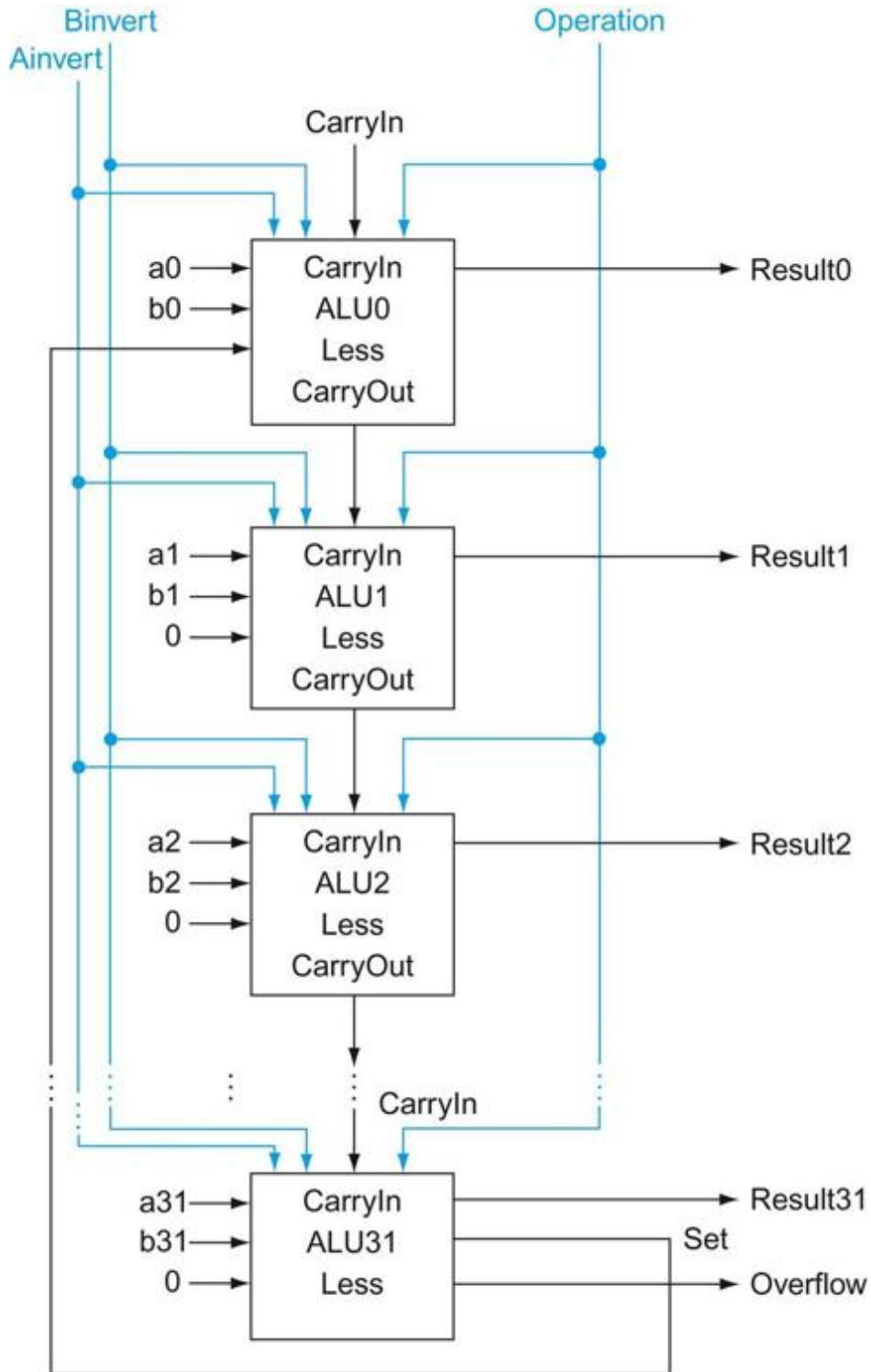
FIGURE B.5.11 A 32-bit ALU constructed from the 31 copies of the 1-bit ALU in the top of Figure B.5.10 and one 1-bit ALU in the bottom of that figure.
