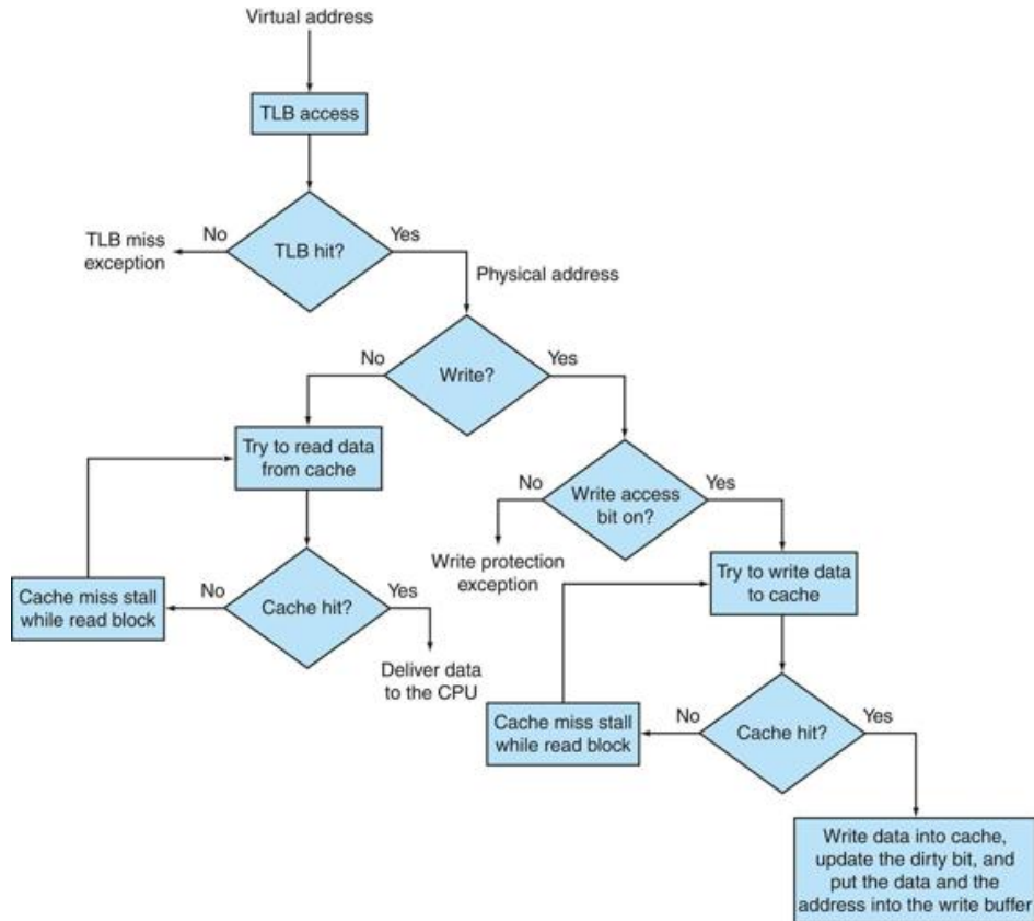
FIGURE 5.30 Processing a read or a write-through in the Intrinsic FastMATH TLB and cache.
