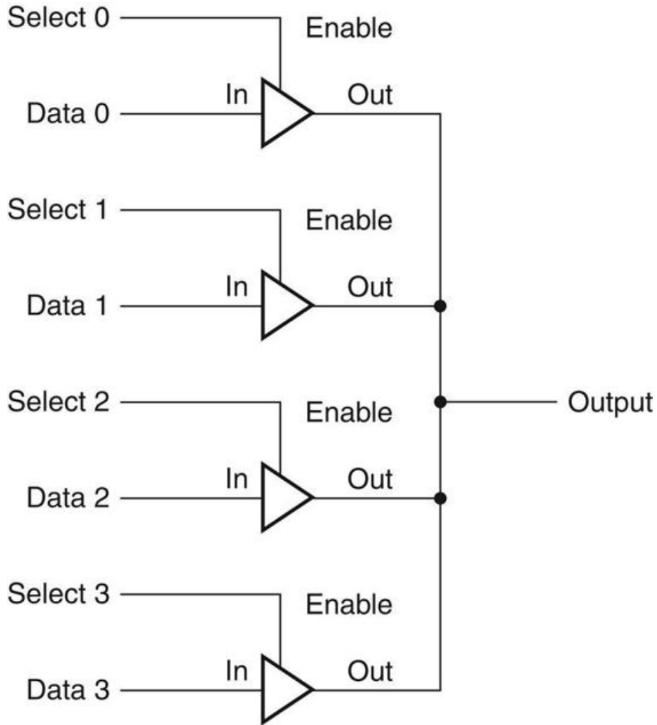
FIGURE B.9.2 Four three-state buffers are used to form a multiplexor.
