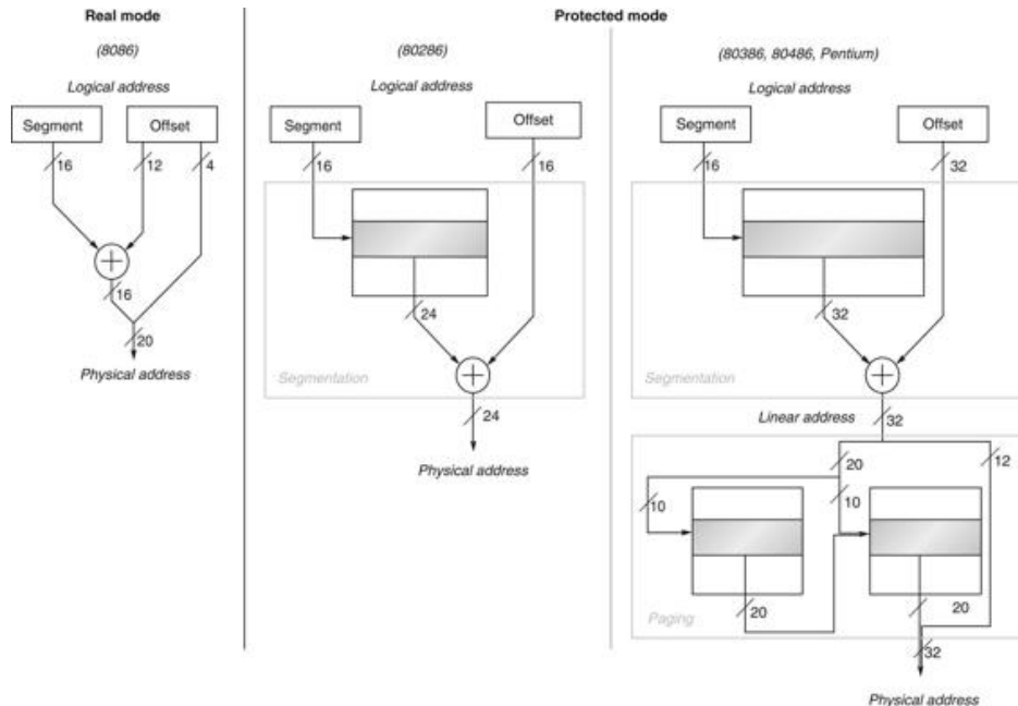
FIGURE E.32 The original segmented scheme of the 8086 is shown on the left.
