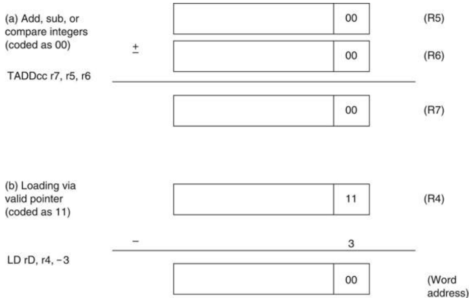
FIGURE E.20 SPARC uses the two least-significant bits to encode different data types for the tagged arithmetic instructions.
