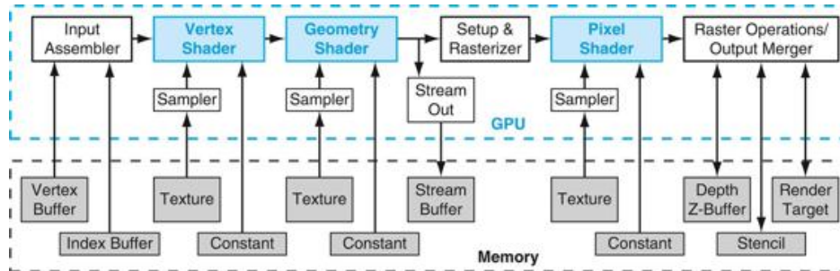
FIGURE C.3.1 Direct3D 10 graphics pipeline.
