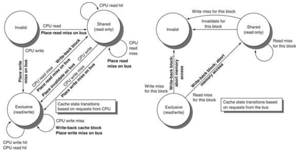
FIGURE E5.12.10 A write-invalidate, cache-coherence protocol for a write-back cache, showing the states and state transitions for each block in the cache.
