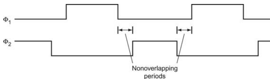
FIGURE B.11.3 A two-phase clocking scheme showing the cycle of each clock and the nonoverlapping periods.
