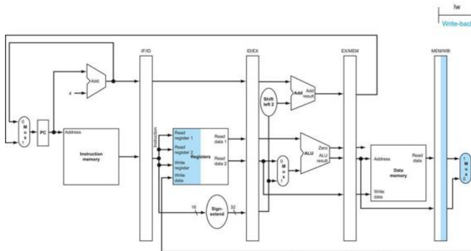
FIGURE 4.38 MEM and WB: The fourth and fifth pipe stages of a load instruction, highlighting the portions of the datapath in Figure 4.35 used in this pipe stage. Data memory is read using the address in the EX/MEM pipeline registers, and the data is placed in the MEM/WB pipeline register. Next, data is read from the MEM/WB pipeline register and written into the register file in the middle of the datapath. Note: there is a bug in this design that is repaired in Figure 4.41 .
