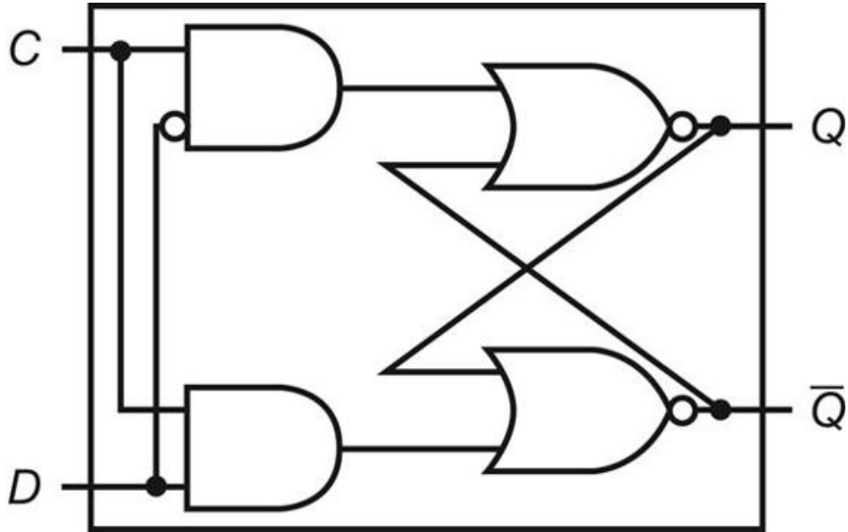
FIGURE B.8.2 A D latch implemented with NOR gates.
