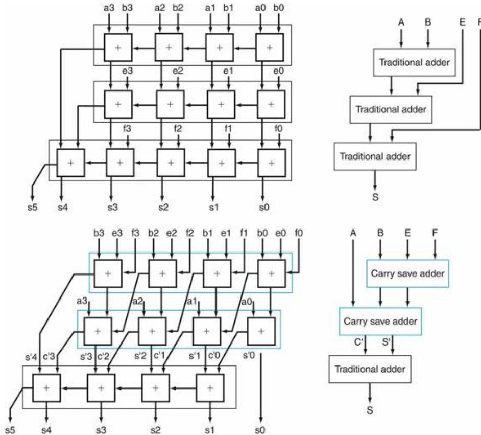
FIGURE B.14.1 Traditional ripple carry and carry save addition of four 4-bit numbers.
