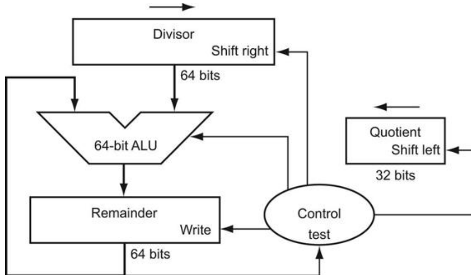
FIGURE 3.8 First version of the division hardware.
