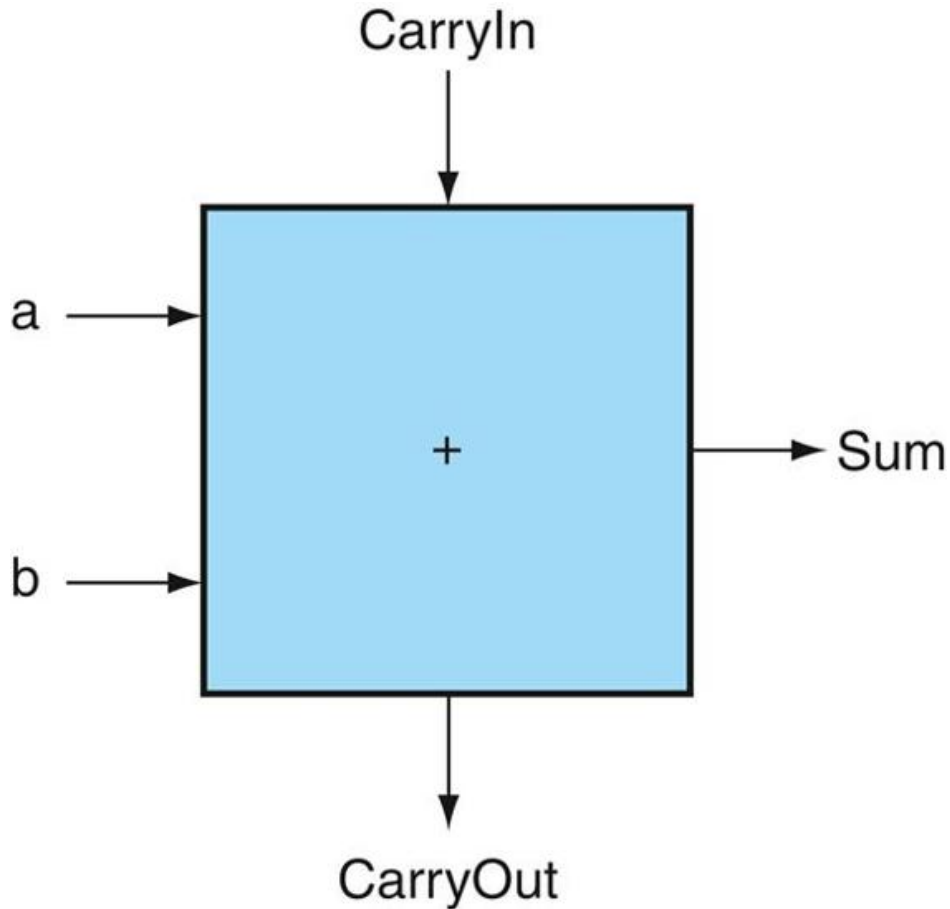
FIGURE B.5.2 A 1-bit adder.
