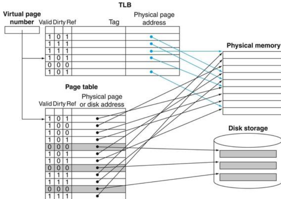
FIGURE 5.28 The TLB acts as a cache of the page table for the entries that map to physical pages only.
