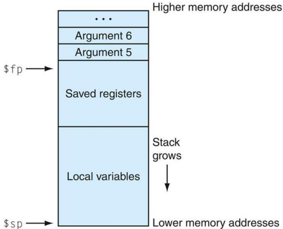
FIGURE A.6.2 Layout of a stack frame.
