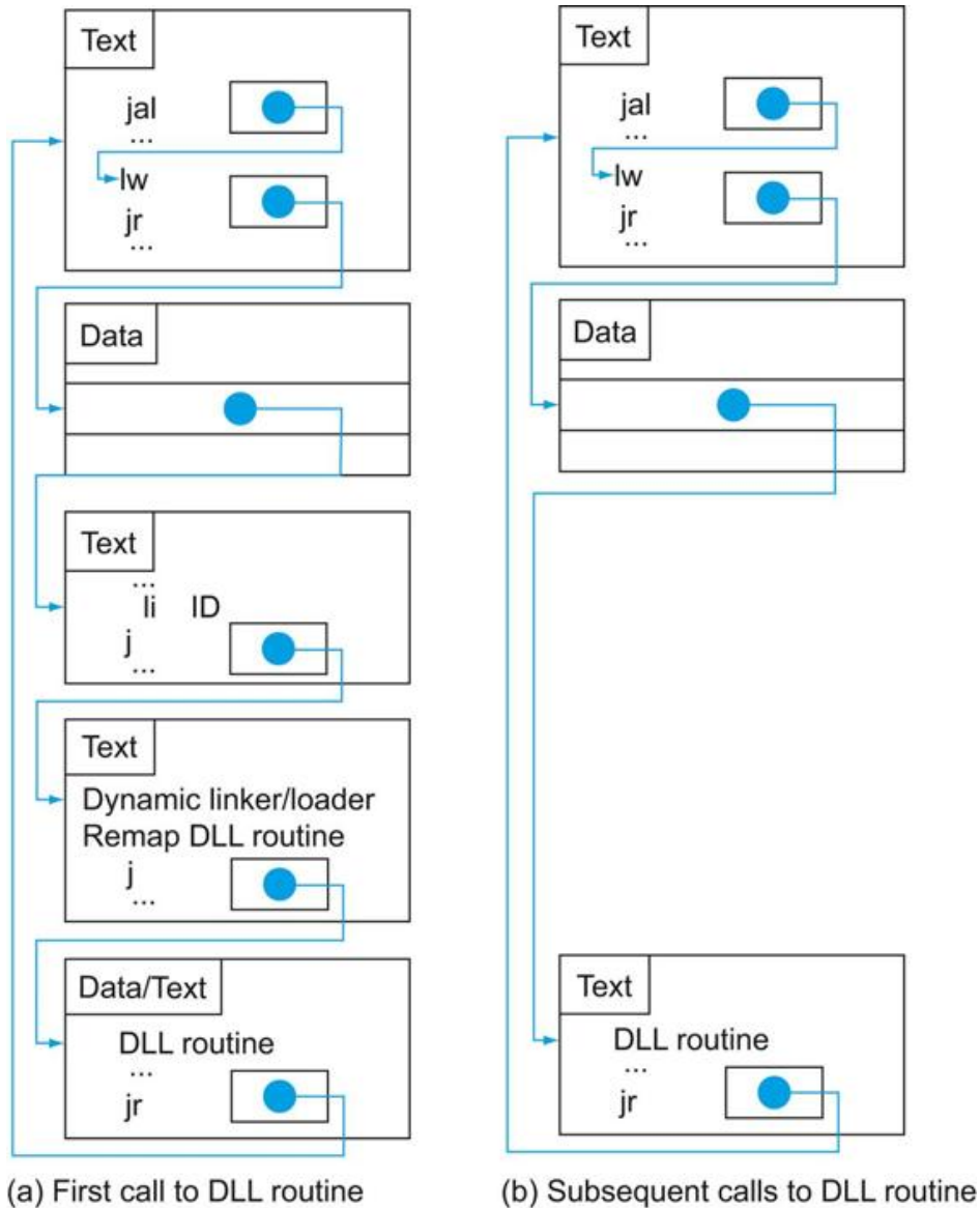
FIGURE 2.22 Dynamically linked library via lazy procedure linkage.
