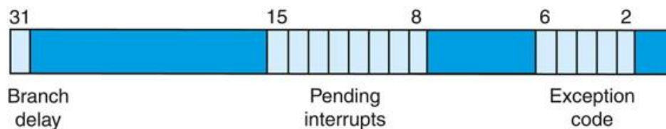
FIGURE A.7.2 The Cause register.
