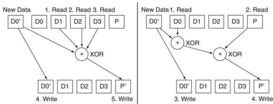
FIGURE E5.11.2 Small write update on RAID 4.
