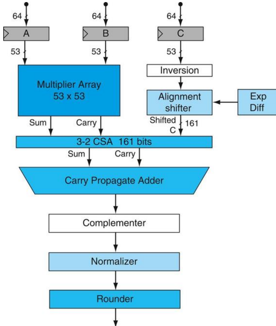
FIGURE C.6.2 Double precision fused-multiply-add (FMA) unit.
