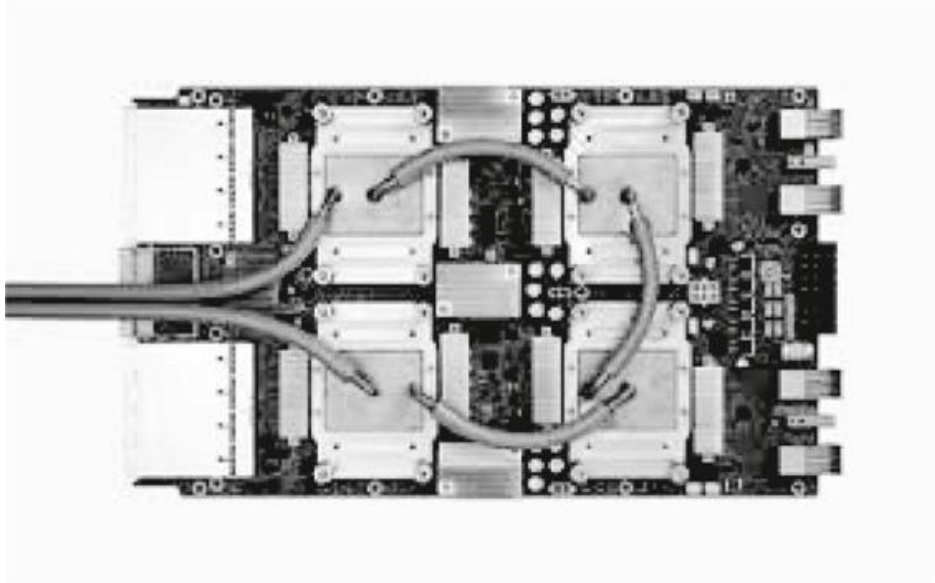
FIGURE 6.24 A TPUv3 supercomputer consisting of up to 1024 chips (left) . It is about 6 ft tall and 40 ft long. A TPUv3 board (right) has four chips and uses liquid cooling.
