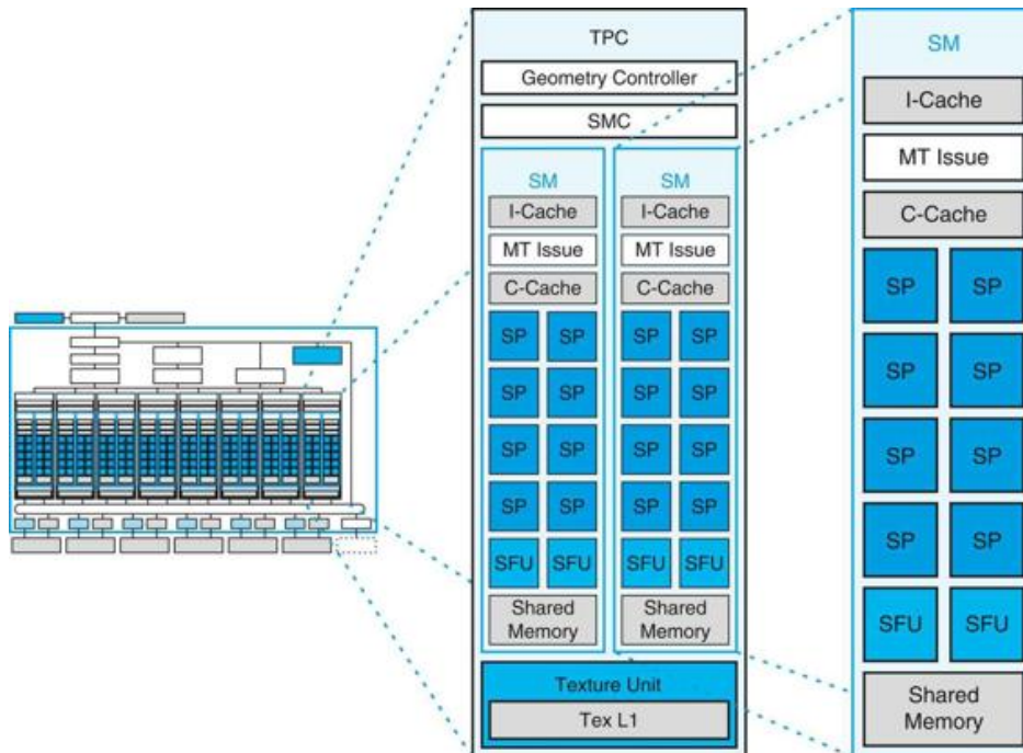
FIGURE C.7.2 Texture/processor cluster (TPC) and a streaming multiprocessor (SM).
