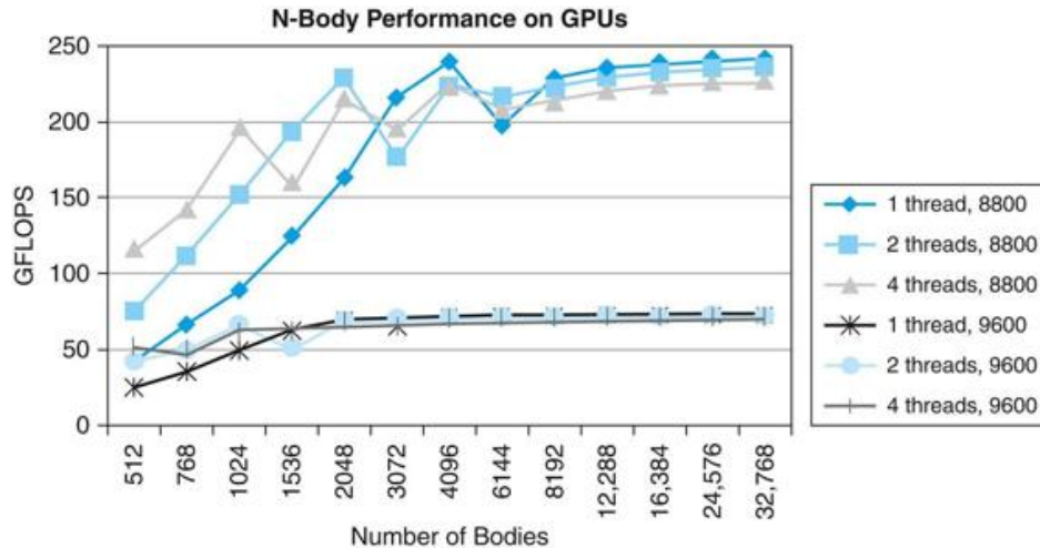
FIGURE C.8.15 Performance measurements of the N-body application on a GeForce 8800 GTX and a GeForce 9600.
