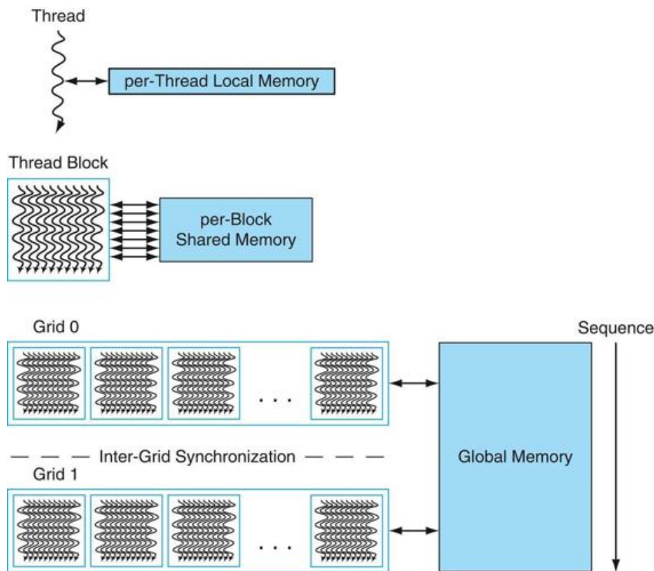
FIGURE C.3.5 Nested granularity levels—thread, thread block, and grid—have corresponding memory sharing levels—local, shared, and global.
