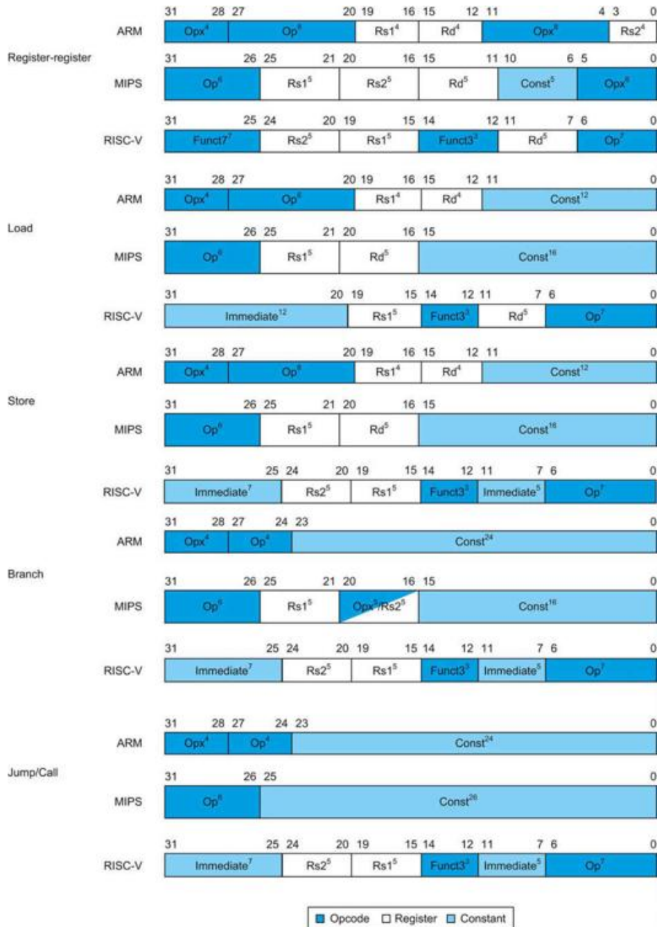
FIGURE 2.34 Instruction formats for ARM, MIPS, and RISC-V.
