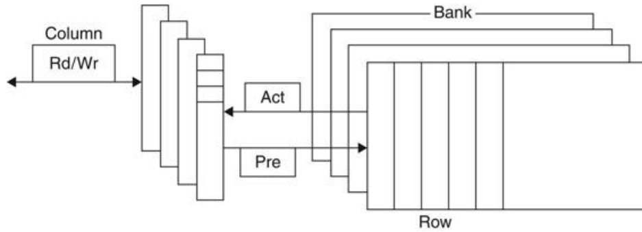
FIGURE 5.4 Internal organization of a DRAM.
