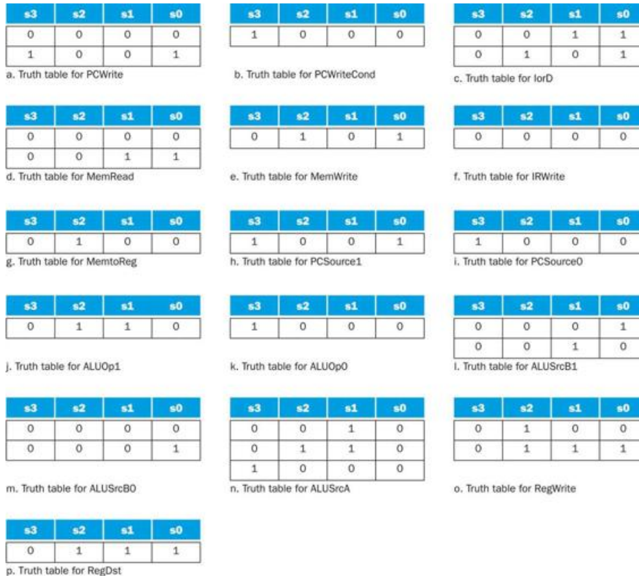
FIGURE D.3.4 The truth tables are shown for the 16 datapath control signals that depend only on the current-state input bits, which are shown for each table.
