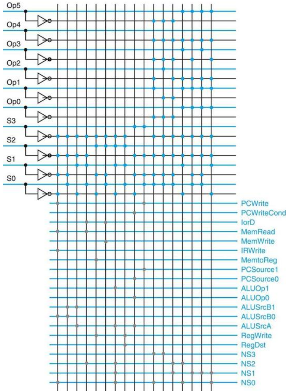
FIGURE D.3.9 This PLA implements the control function logic for the multicycle implementation.
