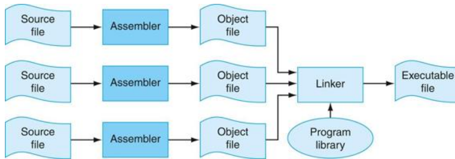
FIGURE A.1.1 The process that produces an executable file.
