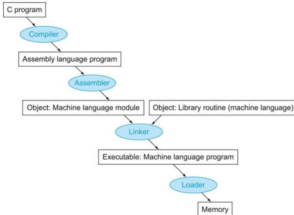
FIGURE 2.21 A translation hierarchy for C.
