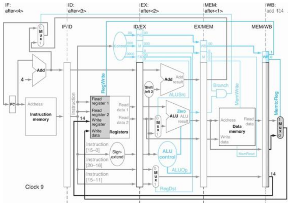
FIGURE E4.14.15 Clock cycle 9.
