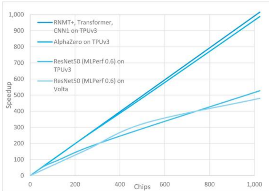
FIGURE 6.29 Supercomputer scaling: TPUv3 and Volta.
