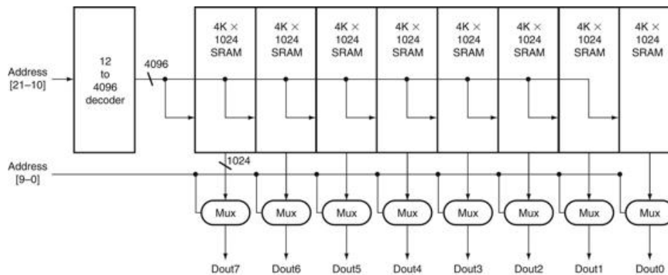
FIGURE B.9.4 Typical organization of a 4\text{M} \times 8 SRAM as an array of 4\text{K} \times 1024 arrays.
