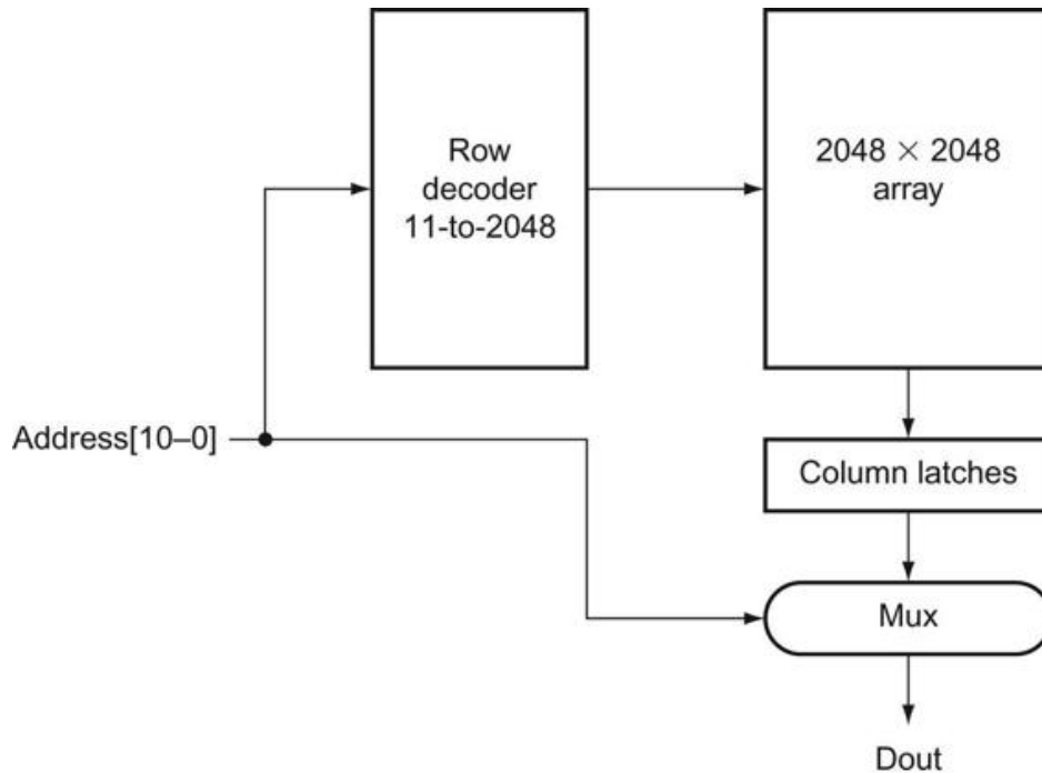
FIGURE B.9.6 A 4\text{M} \times 1 DRAM is built with a 2048 \times 2048 array.
