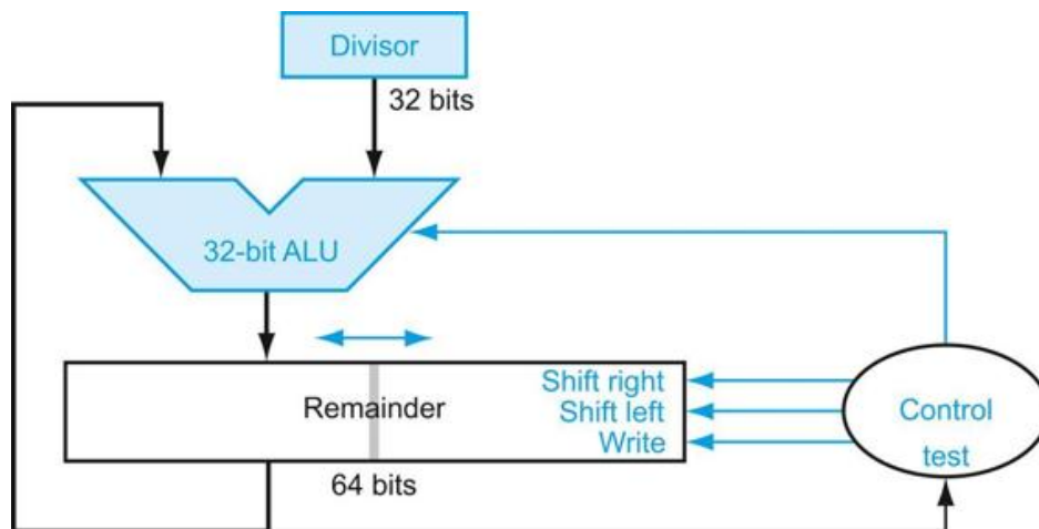
FIGURE 3.11 An improved version of the division hardware.
