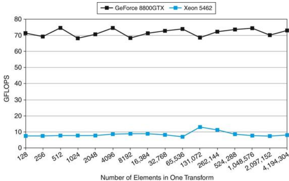
FIGURE C.7.5 Fast Fourier Transform throughput performance.
