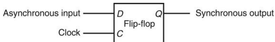
FIGURE B.11.5 A synchronizer built from a D flip-flop is used to sample an asynchronous signal to produce an output that is synchronous with the clock.
