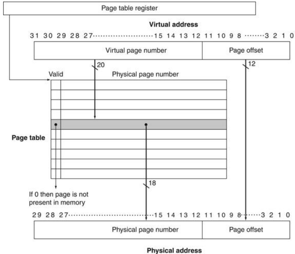
FIGURE 5.26 The page table is indexed with the virtual page number to obtain the corresponding portion of the physical address.
