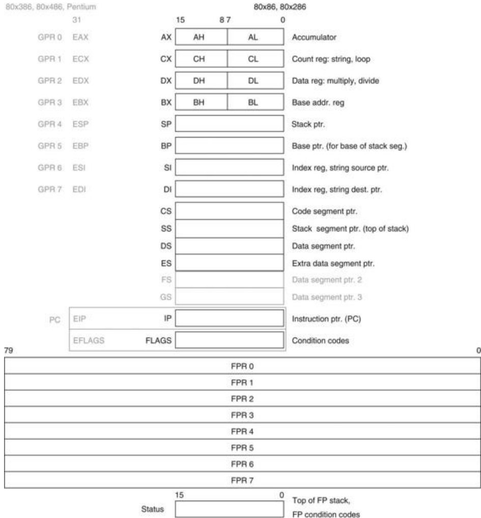
FIGURE E.30 The 80x86 has evolved over time, and so has its register set.
