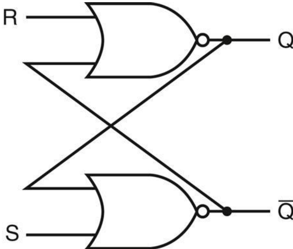
FIGURE B.8.1 A pair of cross-coupled NOR gates can store an internal value.
