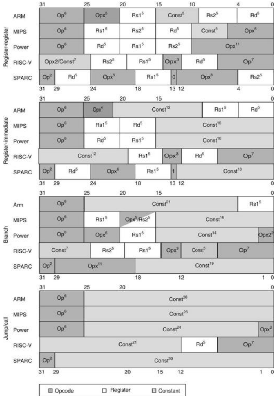
FIGURE E.6 Instruction formats for desktop/server RISC architectures. These four formats are found in all five architectures.
