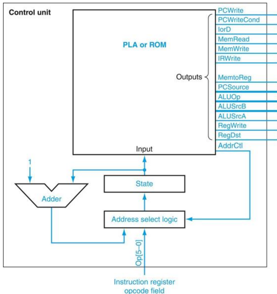
FIGURE D.4.1 The control unit using an explicit counter to compute the next state.
