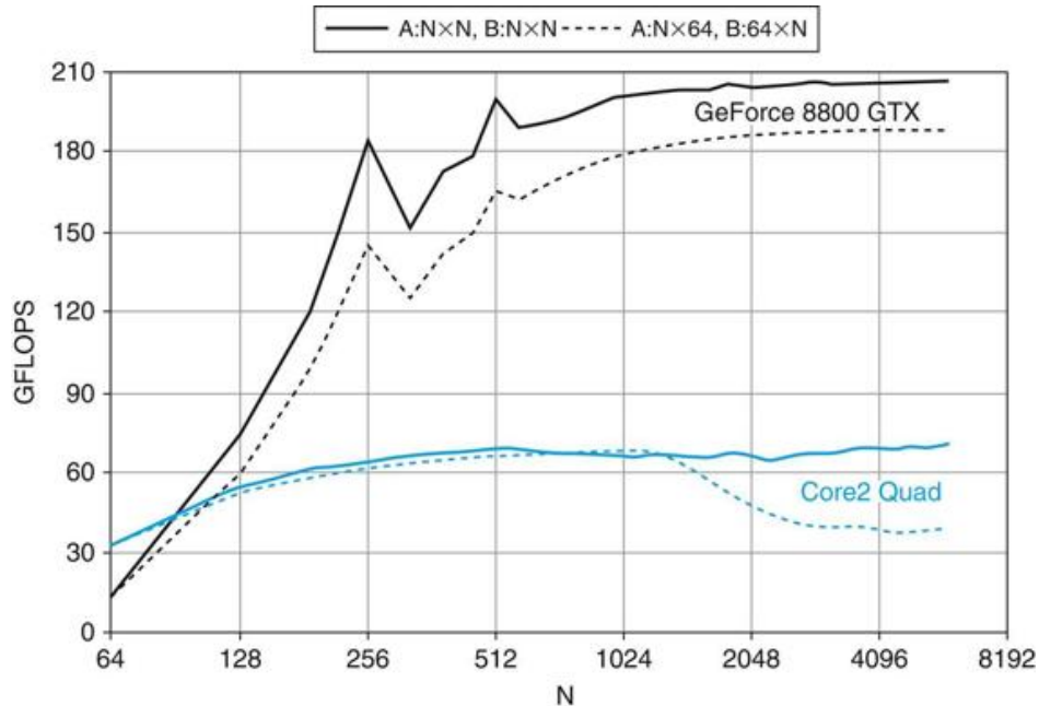
FIGURE C.7.3 SGEMM dense matrix-matrix multiplication performance rates.
