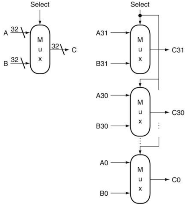
a. A 32-bit wide 2-to-1 multiplexor
