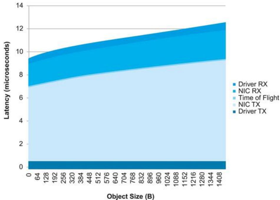
FIGURE E6.10.4 Time to send an object broken into transmit driver and NIC hardware time vs. receive driver and NIC hardware time.
