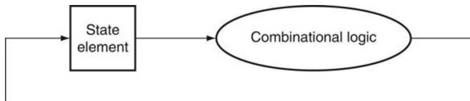
FIGURE B.7.3 An edge-triggered methodology allows a state element to be read and written in the same clock cycle without creating a race that could lead to undetermined data values.
