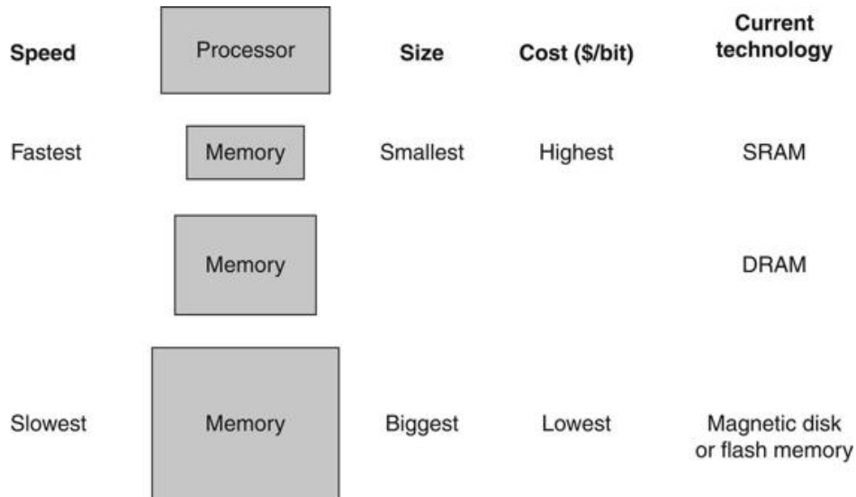
FIGURE 5.1 The basic structure of a memory hierarchy.
