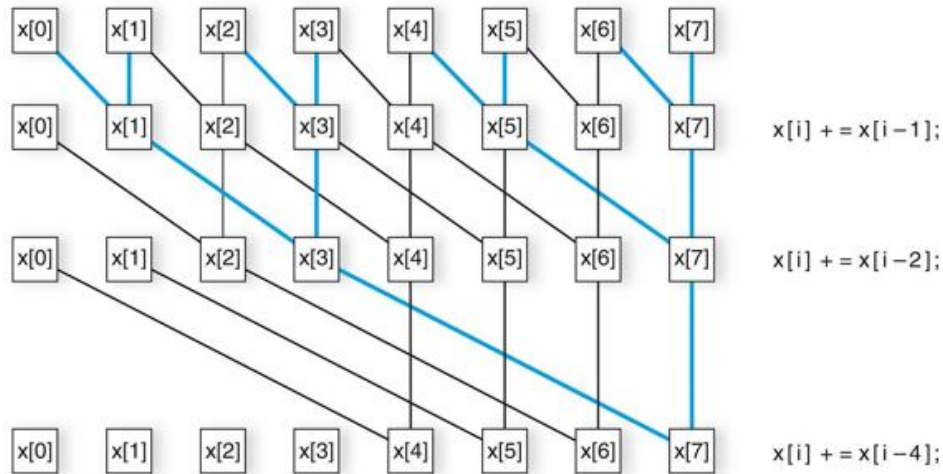
FIGURE C.8.8 Tree-based parallel scan data references.
