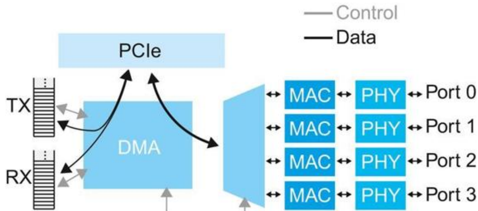
FIGURE E6.10.2 Block diagram of the NetFPGA Ethernet card in Figure e6.10.1 showing the control paths and the data paths.
