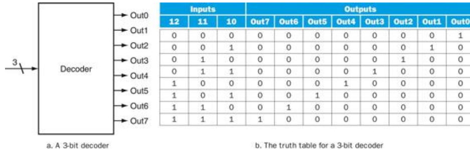
FIGURE B.3.1 A 3-bit decoder has 3 inputs, called 12, 11, and 10, and 2^3 = 8 outputs, called Out0 to Out7.
