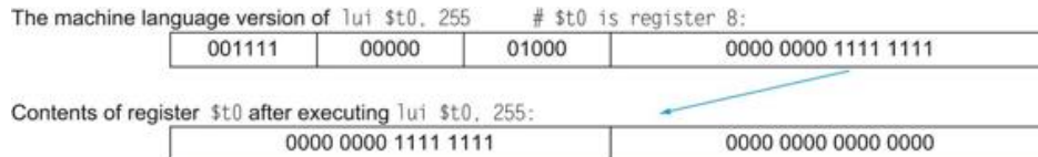
FIGURE 2.17 The effect of the lui instruction.
