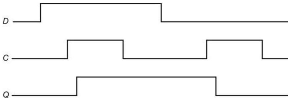
FIGURE B.8.3 Operation of a D latch, assuming the output is initially deasserted.
