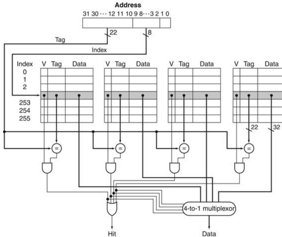
FIGURE 5.18 The implementation of a four-way set-associative cache requires four comparators and a 4-to-1 multiplexor.
