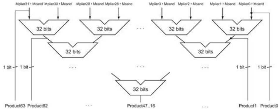
FIGURE 3.7 Fast multiplication hardware.
