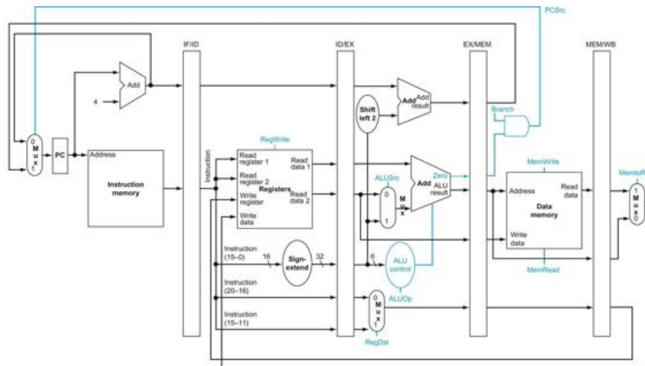
FIGURE 4.46 The pipelined datapath of Figure 4.41 with the control signals identified.
