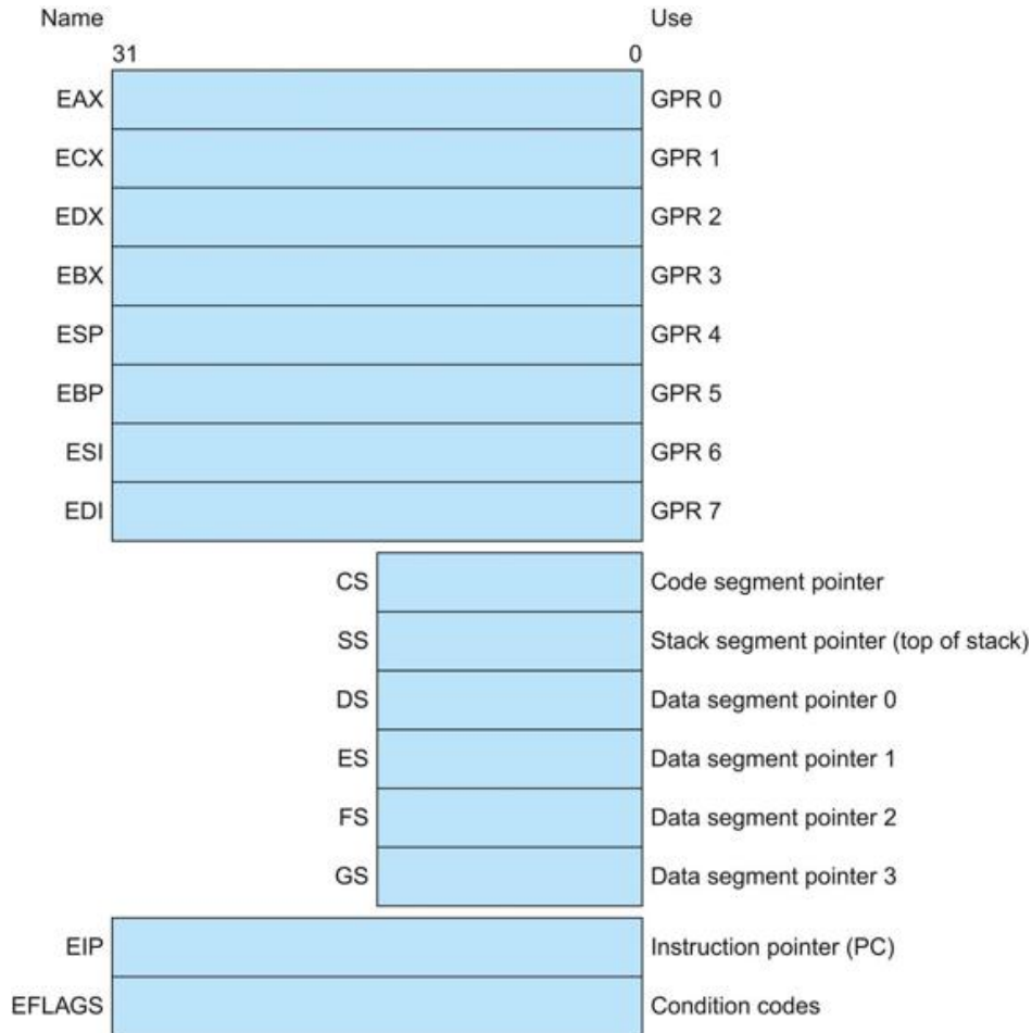
FIGURE 2.36 The 80386 register set.
