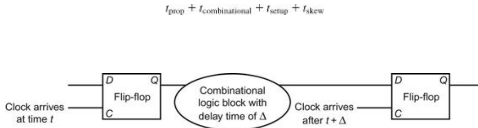
FIGURE B.11.2 Illustration of how clock skew can cause a race, leading to incorrect operation.
