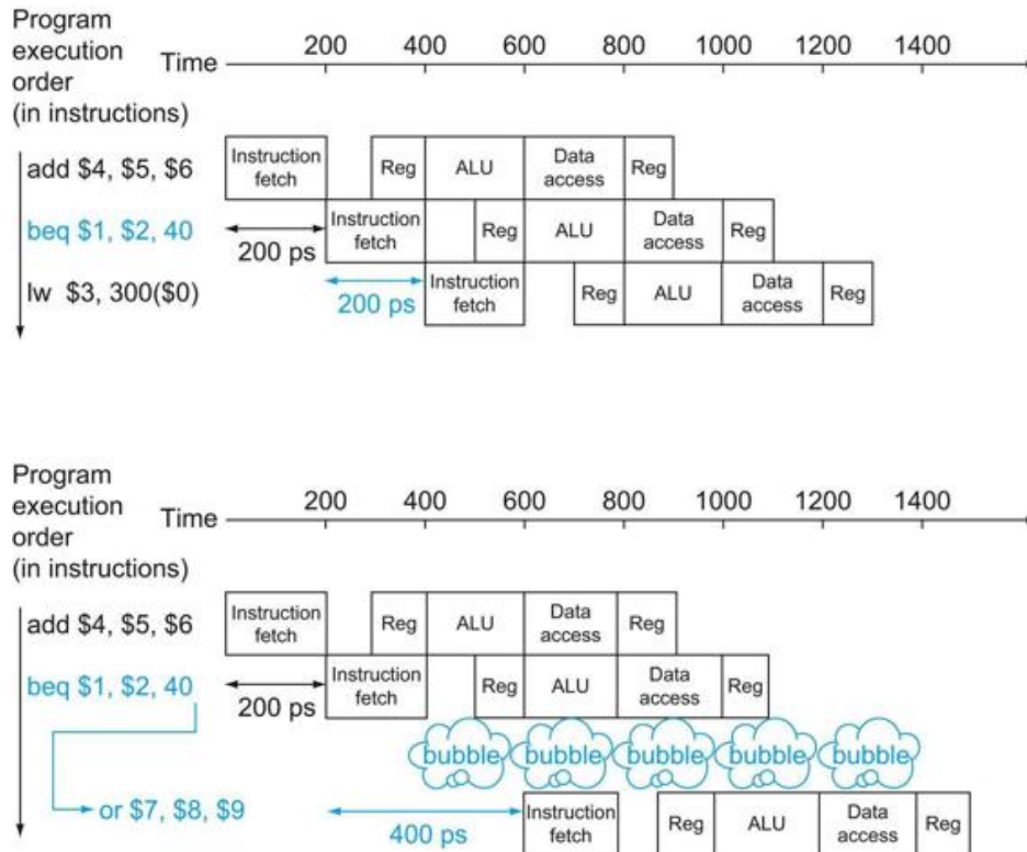
FIGURE 4.32 Predicting that branches are not taken as a solution to control hazard.
