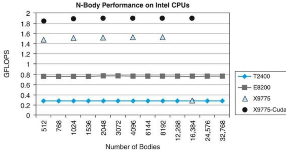
FIGURE C.8.16 Performance measurements on the N-body code on a CPU.
