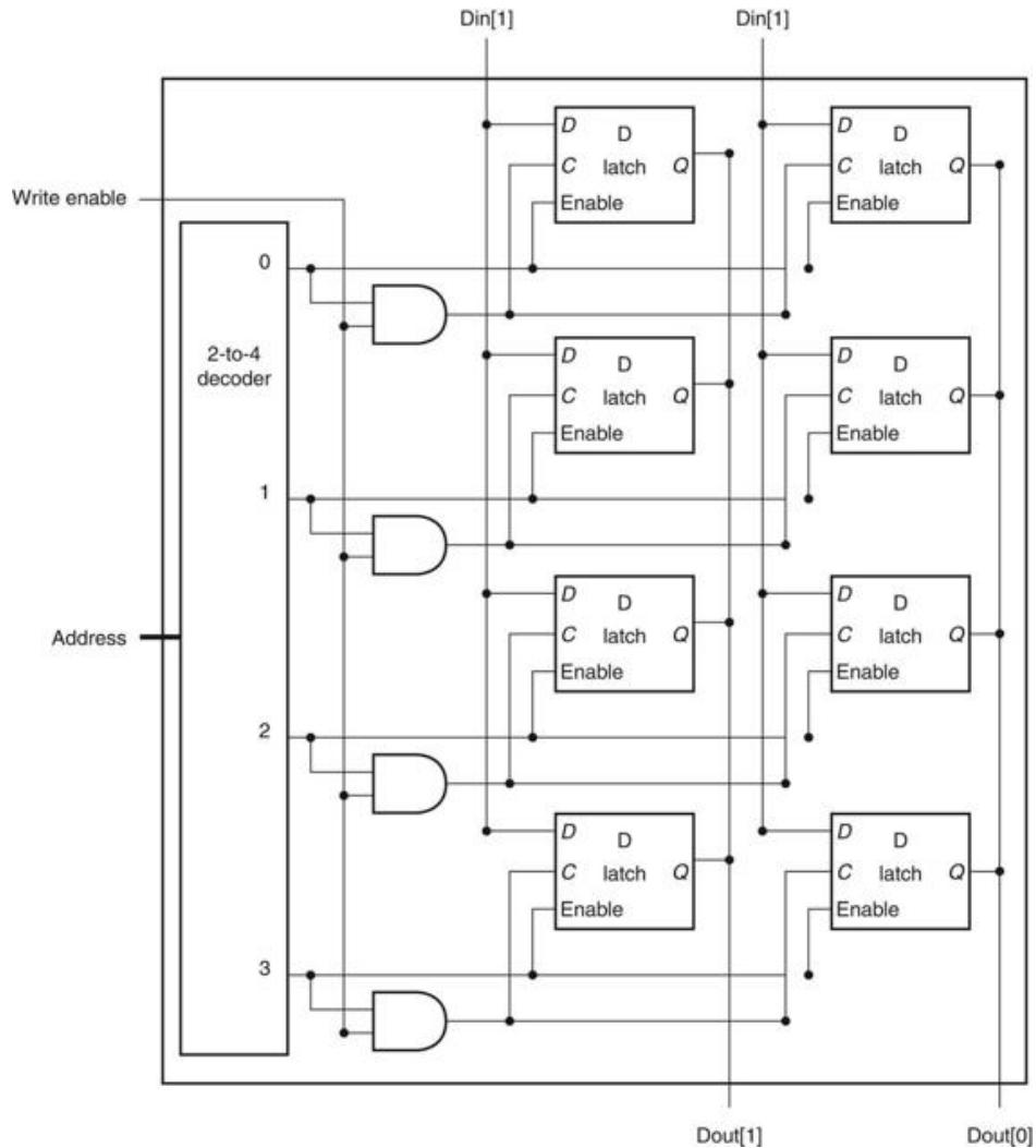
FIGURE B.9.3 The basic structure of a 4 \times 2 SRAM consists of a decoder that selects which pair of cells to activate.
