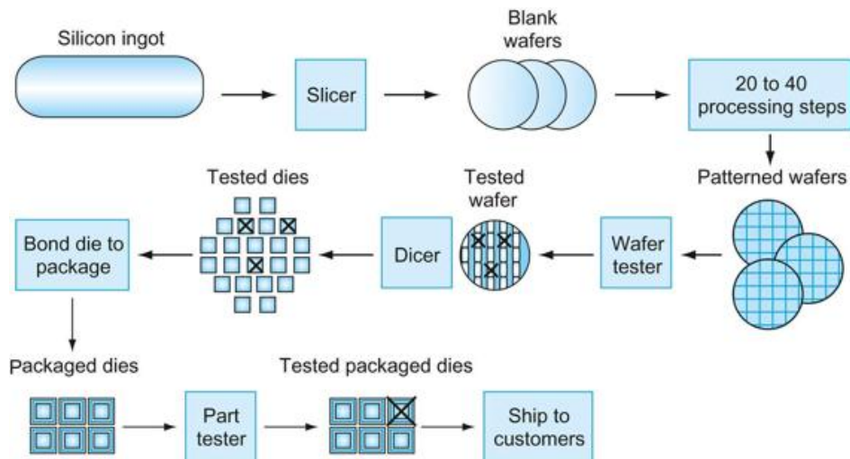
FIGURE 1.12 The chip manufacturing process.
