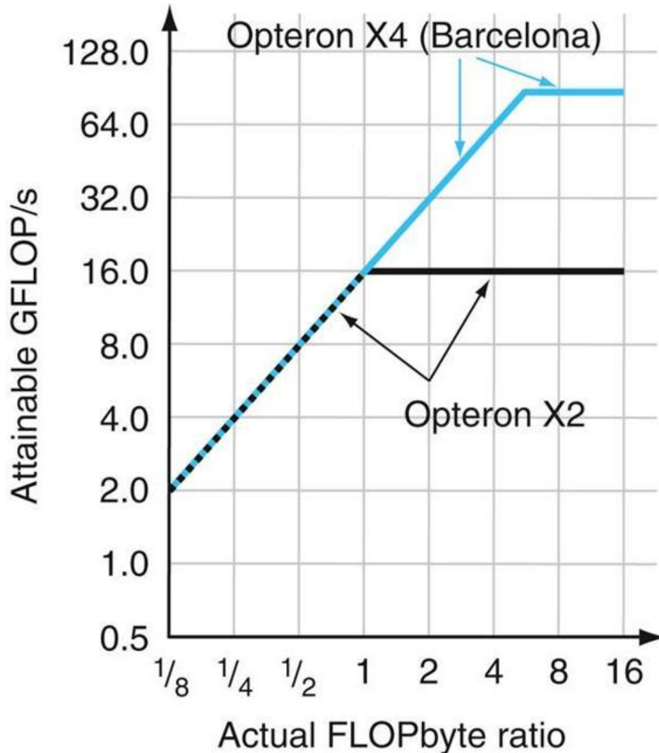
FIGURE 6.20 Roofline models of two generations of Opterons.
