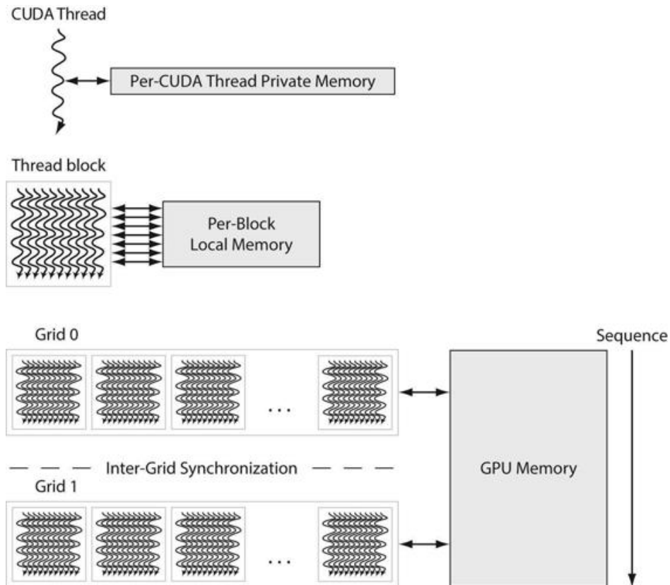
FIGURE 6.10 GPU Memory structures.
