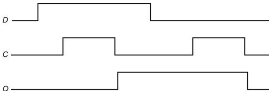
FIGURE B.8.5 Operation of a D flip-flop with a falling-edge trigger, assuming the output is initially deasserted.
