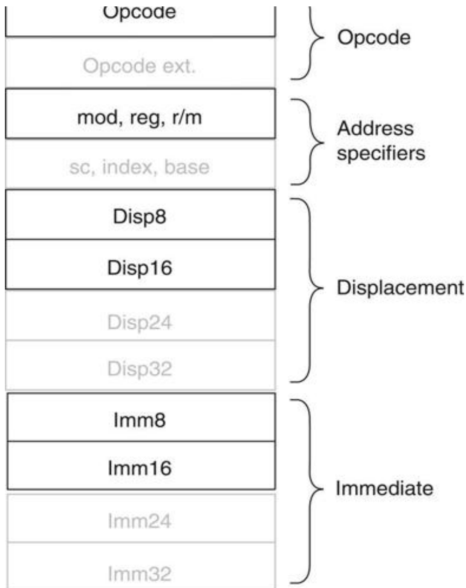
FIGURE E.36 The instruction format of the 8086 (black type) and the extensions for the 80386 (shaded type). Every field is optional except the opcode.
