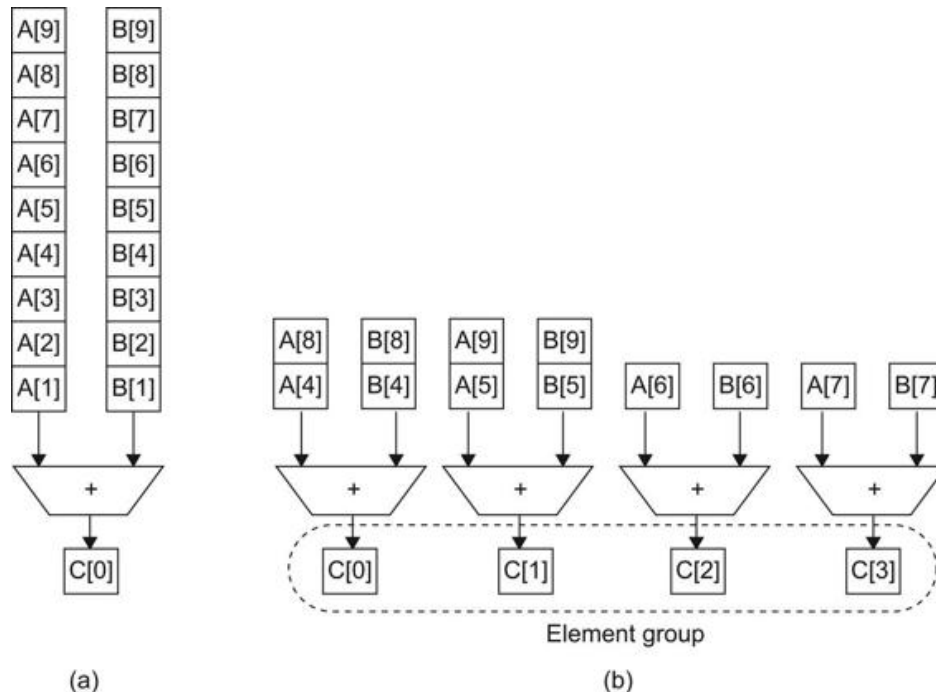
FIGURE 6.3 Using multiple functional units to improve the performance of a single vector add instruction, C = A + B .
