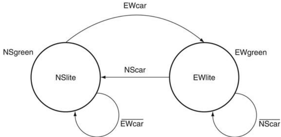
FIGURE B.10.2 The graphical representation of the two-state traffic light controller.
