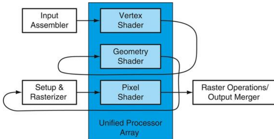
FIGURE C.2.4 Logical pipeline mapped to physical processors.
