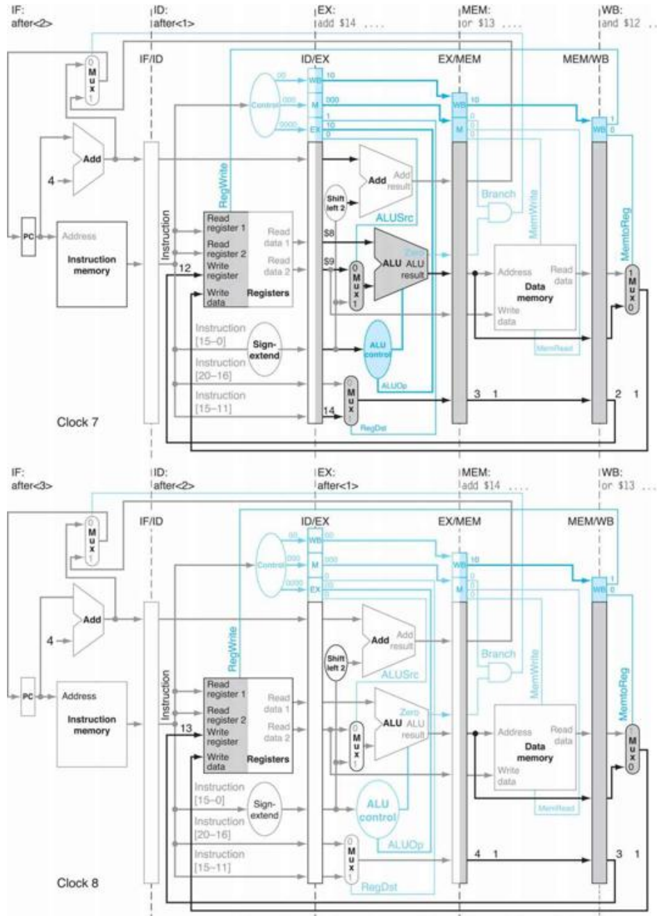
FIGURE E4.14.14 Clock cycles 7 and 8.
