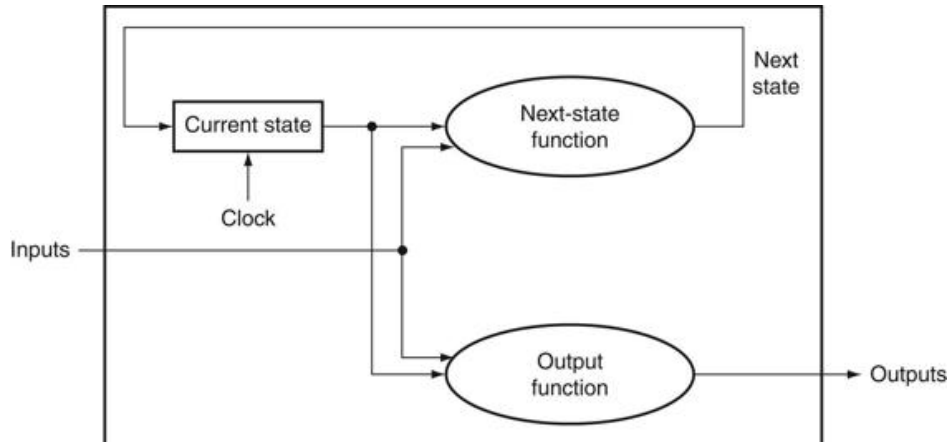
FIGURE B.10.1 A state machine consists of internal storage that contains the state and two combinational functions: the next-state function and the output function.
