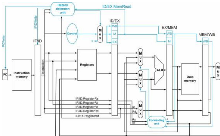
FIGURE 4.60 Pipelined control overview, showing the two multiplexers for forwarding, the hazard detection unit, and the forwarding unit.
