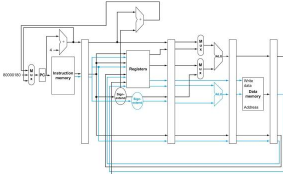
FIGURE 4.69 A static two-issue datapath.
