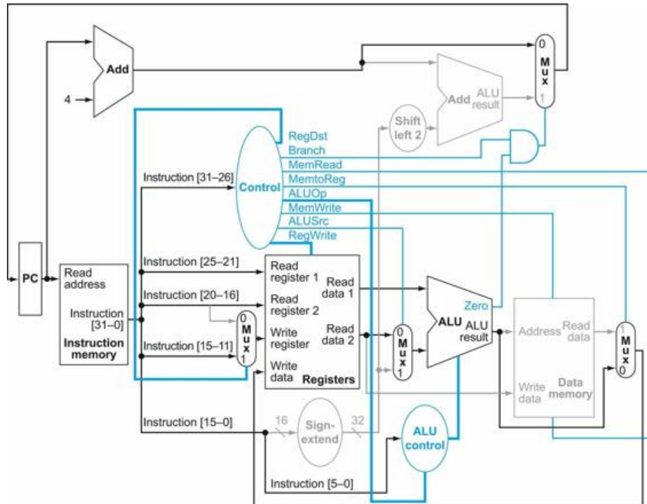
FIGURE 4.19 The datapath in operation for an R-type instruction, such as add $t1, $t2, $t3 .
