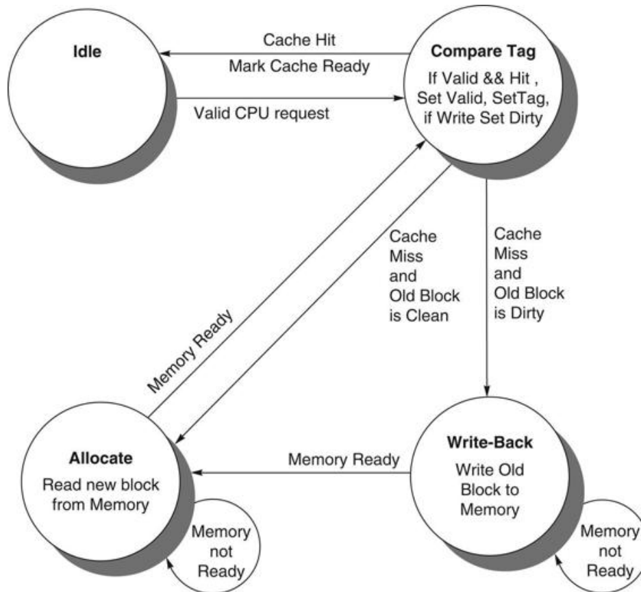
FIGURE 5.39 Four states of the simple controller.
