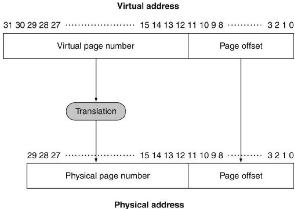
FIGURE 5.25 Mapping from a virtual to a physical address.
