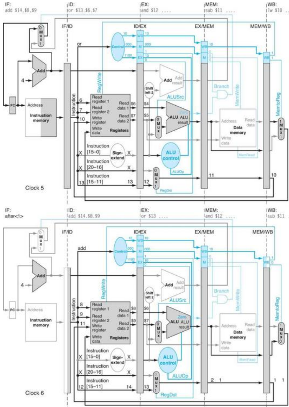
FIGURE E4.14.13 Clock cycles 5 and 6.
