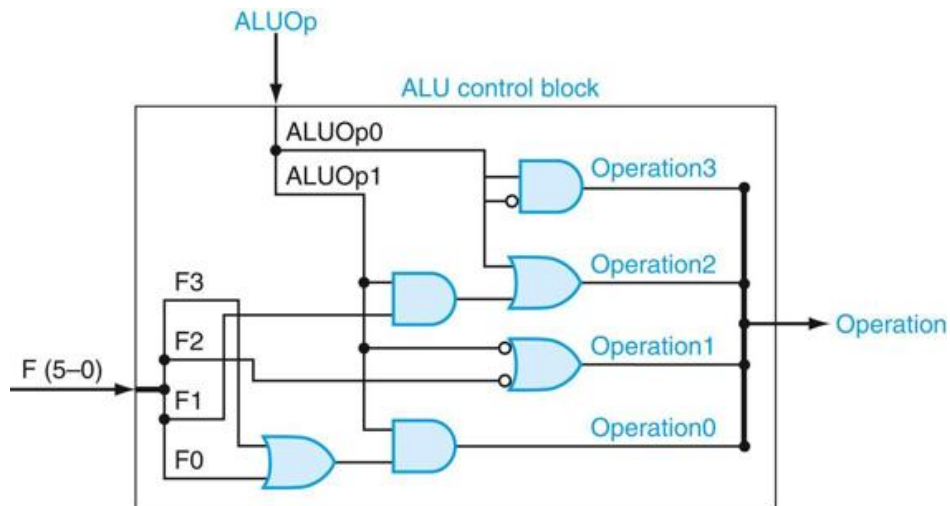
FIGURE D.2.3 The ALU control block generates the four ALU control bits, based on the function code and ALUOp bits.
