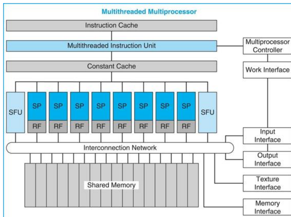
FIGURE C.4.1 Multithreaded multiprocessor with eight scalar processor (SP) cores.
