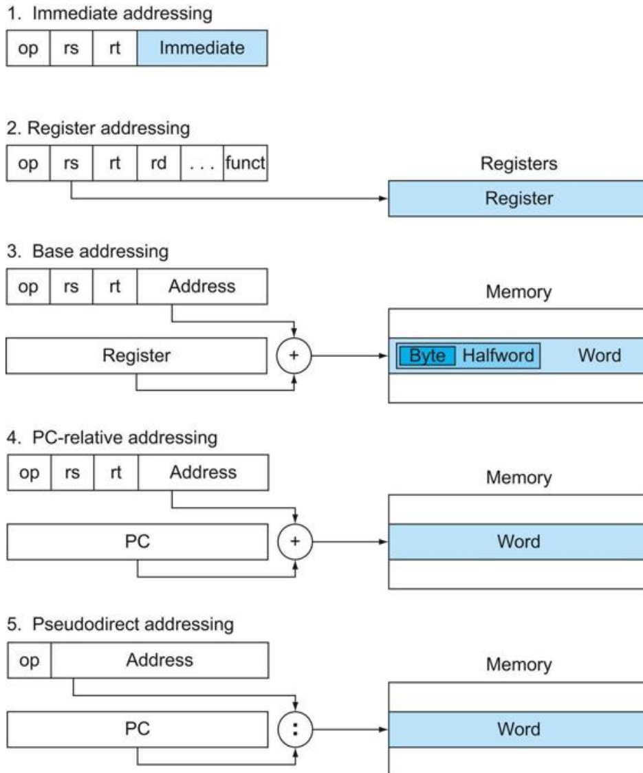
FIGURE 2.18 Illustration of the five MIPS addressing modes.
