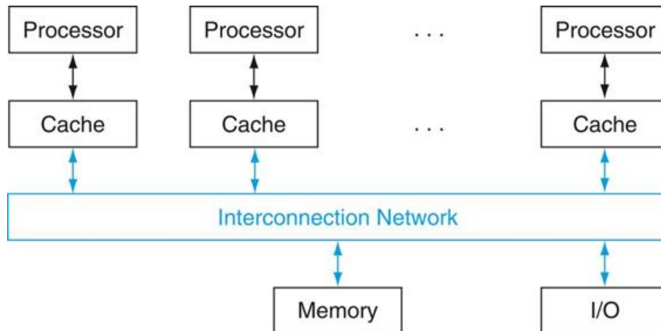
FIGURE 6.7 Classic organization of a shared memory multiprocessor.
