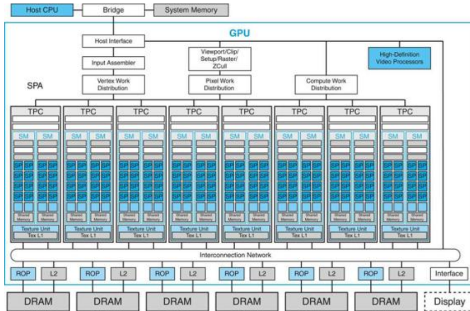
FIGURE C.7.1 NVIDIA Tesla unified graphics and computing GPU architecture.
