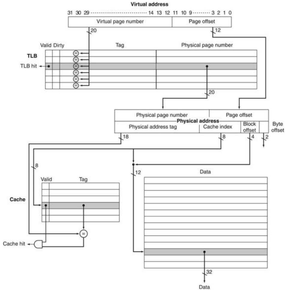
FIGURE 5.29 The TLB and cache implement the process of going from a virtual address to a data item in the Intrinsic FastMATH.
