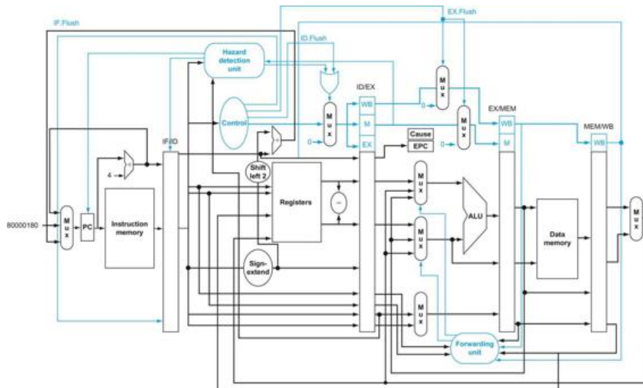
FIGURE 4.66 The datapath with controls to handle exceptions.
