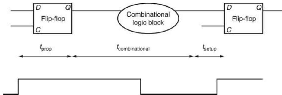
FIGURE B.11.1 In an edge-triggered design, the clock must be long enough to allow signals to be valid for the required setup time before the next clock edge.
