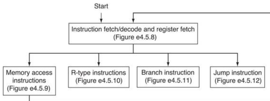
FIGURE E4.5.7 The high-level view of the finite-state machine control.
