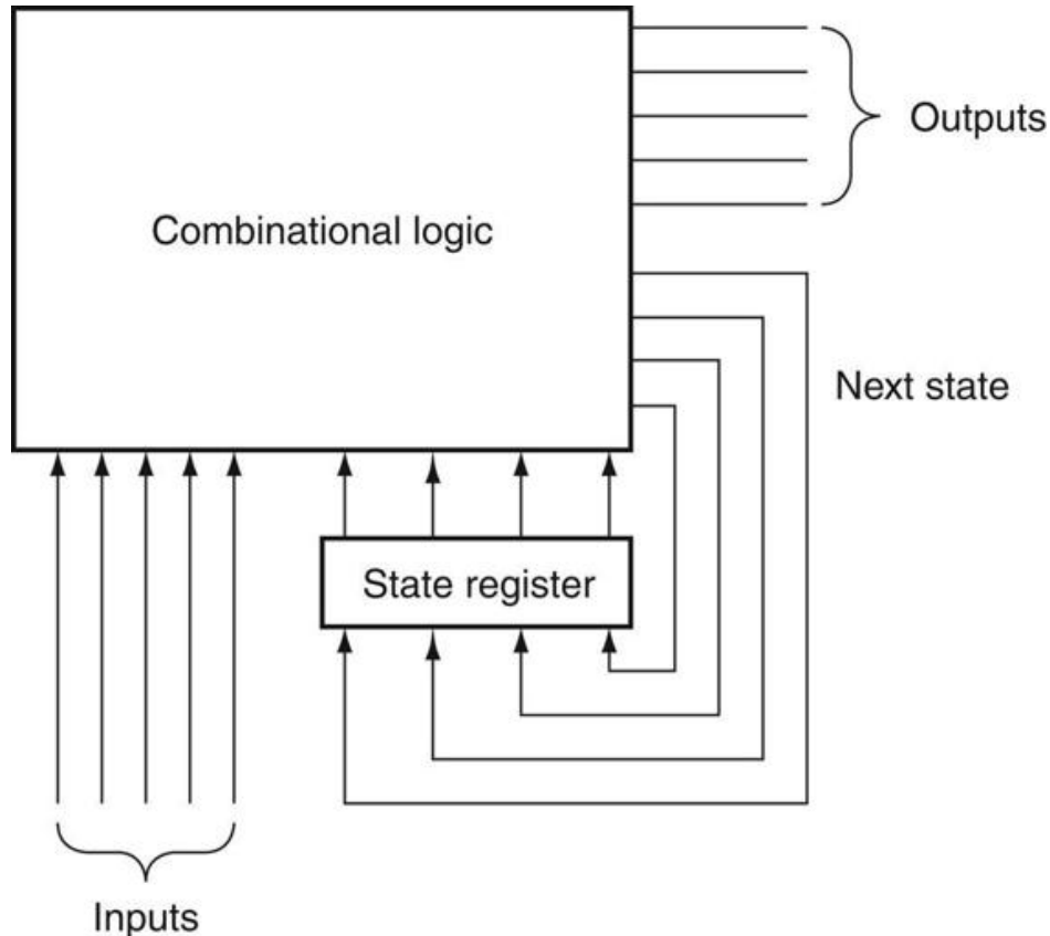
FIGURE B.10.3 A finite-state machine is implemented with a state register that holds the current state and a combinational logic block to compute the next state and output functions.
