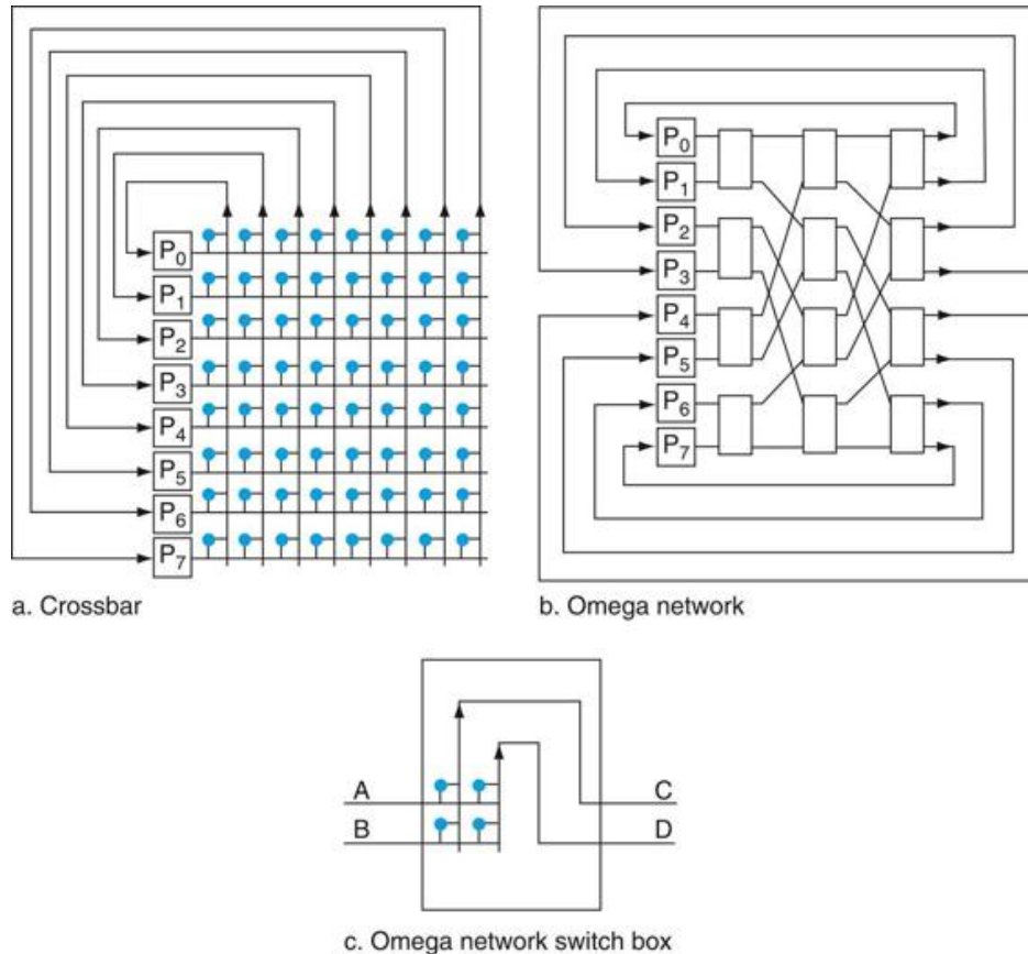
FIGURE 6.16 Popular multistage network topologies for eight nodes.
