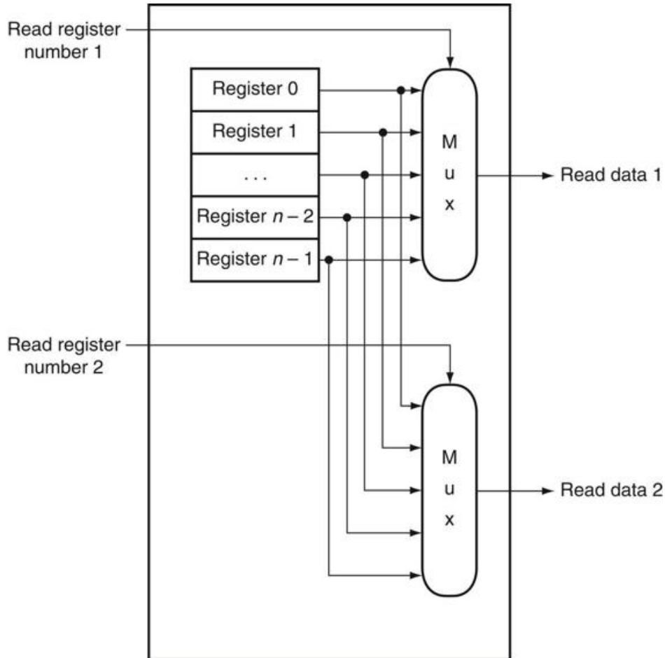
FIGURE B.8.8 The implementation of two read ports for a register file with n registers can be done with a pair of n -to-1 multiplexers, each 32 bits wide.
