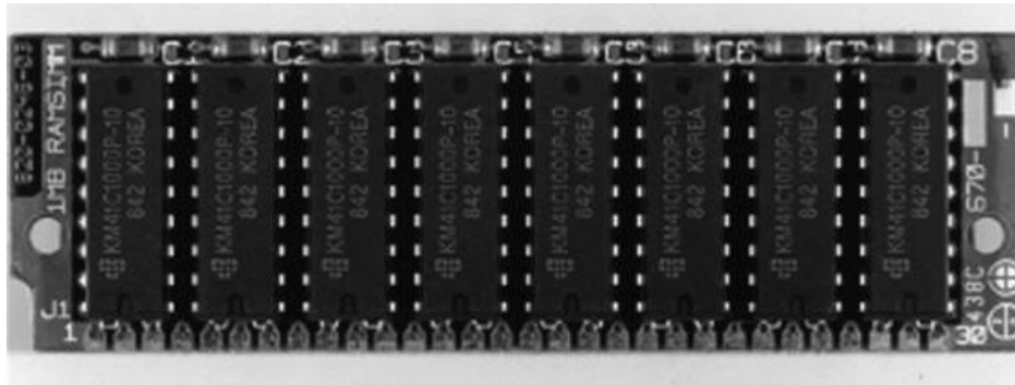
FIGURE E5.17.4 A 1 MB SIMM, built in 1986, using 1 Mbit chips.
