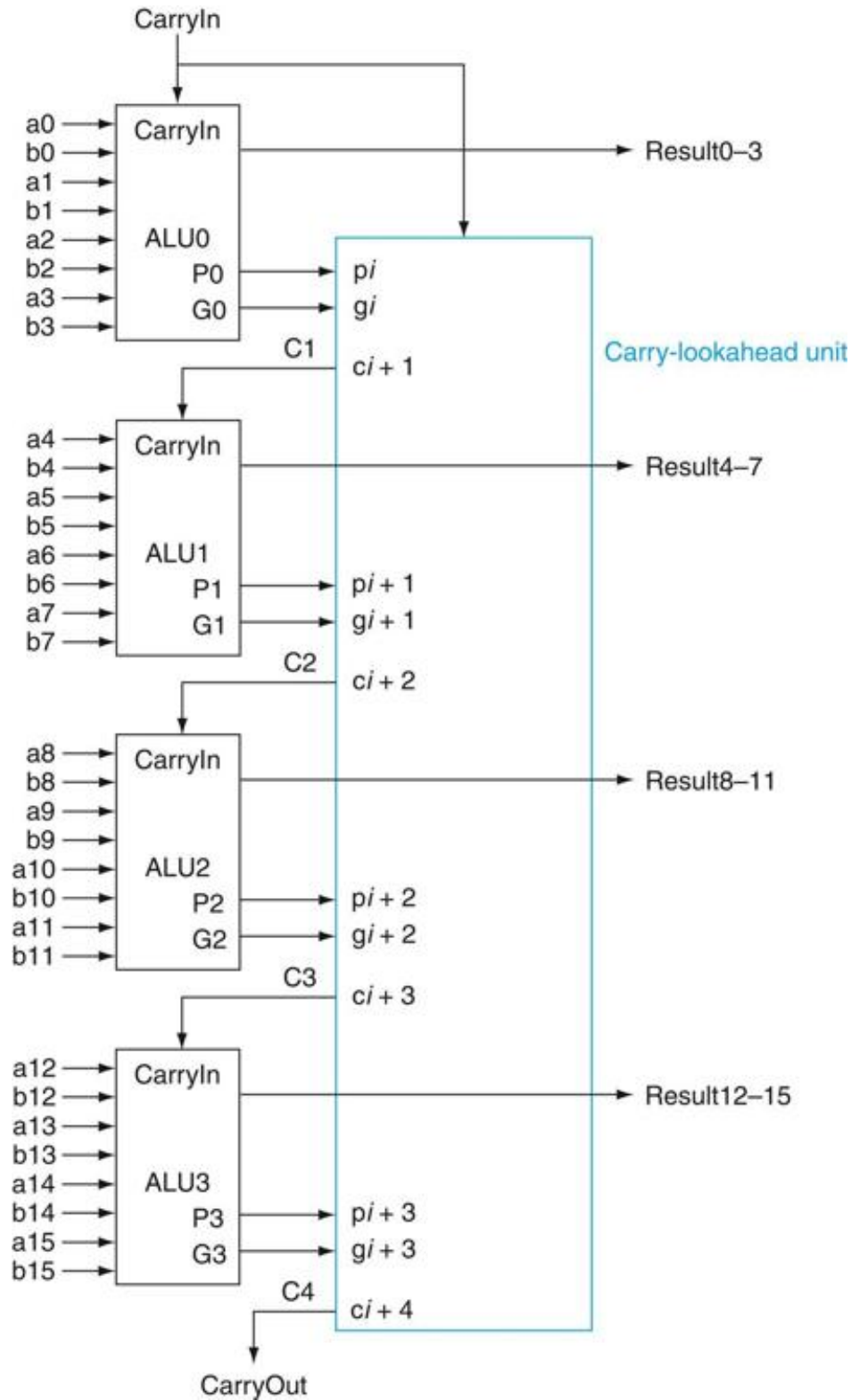
FIGURE B.6.3 Four 4-bit ALUs using carry lookahead to form a 16-bit adder.
