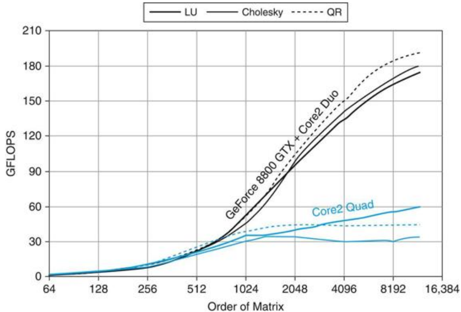
FIGURE C.7.4 Dense matrix factorization performance rates.
