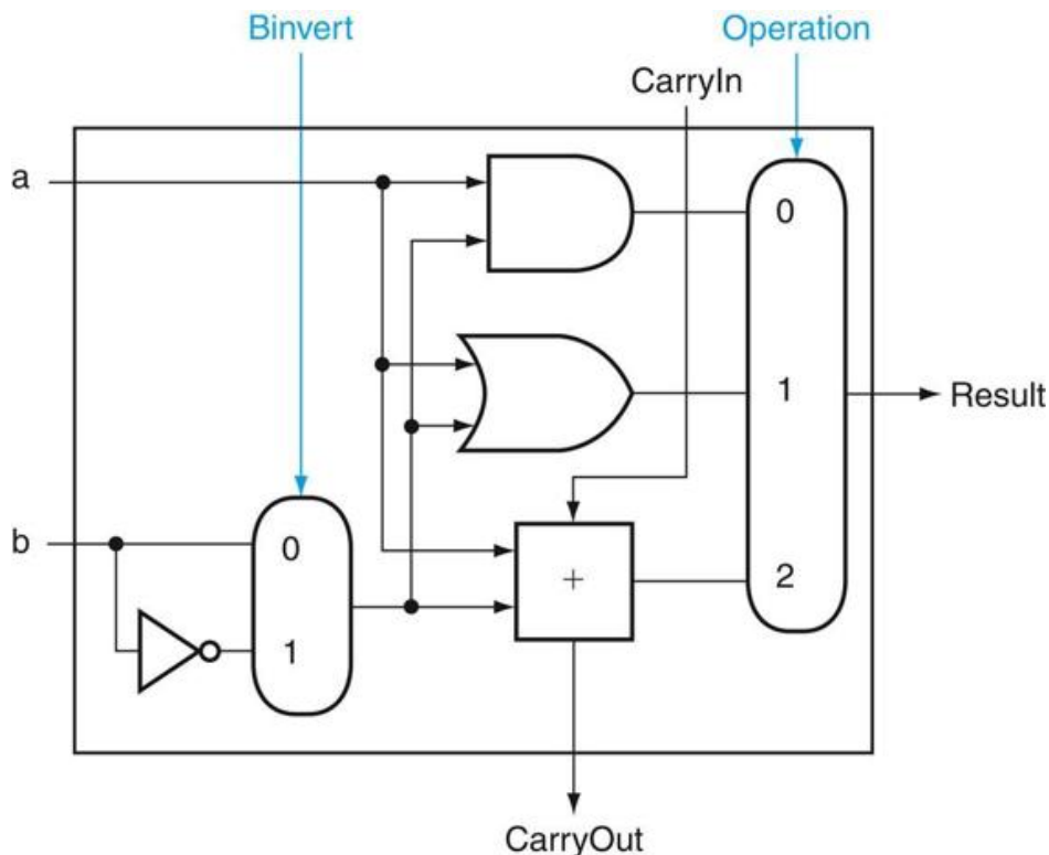
FIGURE B.5.8 A 1-bit ALU that performs AND, OR, and addition on a and b or a and \bar{b} .
