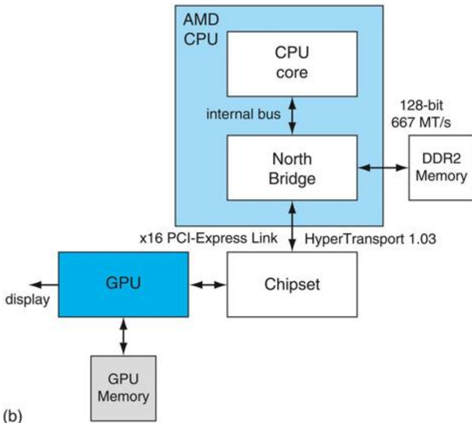
FIGURE C.2.2 Contemporary PCs with Intel and AMD CPUs.
