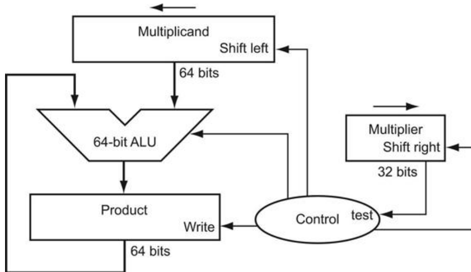
FIGURE 3.3 First version of the multiplication hardware.
